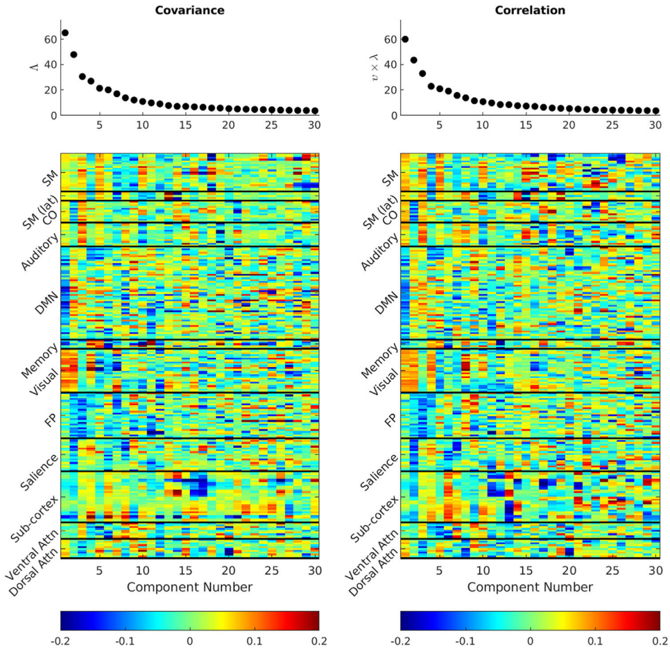
Fig. 3. Principal component analysis of \widehat{\mathbf{C}}_{\text{CONT}} and correlation \widehat{\mathbf{r}}_{\text{CONT}} matrices obtained in the control participants. Scree plots are shown above corresponding eigenvectors. The correlation eigenvectors have been multiplied by the scalar constant ( \nu_{\text{CONT}} = 2.98 ) that minimizes error in the proportionality model, \langle \widehat{\mathbf{C}}_{\text{CONT}} \rangle_{\mathbf{k}} = \nu_{\text{CONT}} \langle \widehat{\mathbf{r}}_{\text{CONT}} \rangle_{\mathbf{k}} . The first few eigenvectors exhibit clustered, large loadings within resting state networks, e.g., the DMN. Network structure becomes fragmented at higher eigenvector indices in both the covariance and correlation representations of FC.
