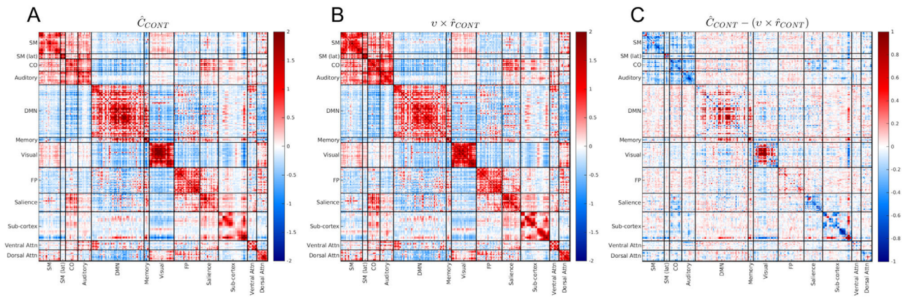
Fig. 4. Blockwise scalar proportionality between covariance and correlation matrices in the control population. Panel A shows \hat{C}_{CONT} . Panel B shows v_{CONT} \hat{f}_{CONT} . Panel C shows the difference, \hat{C}_{CONT} - v_{CONT} \hat{f}_{CONT} , i.e., focal deviations from block-wise scalar proportionality. These deviations account for only 6% of total variance ( \eta_{CONT}^2 = 0.94 ). Note scale change in panel C.
