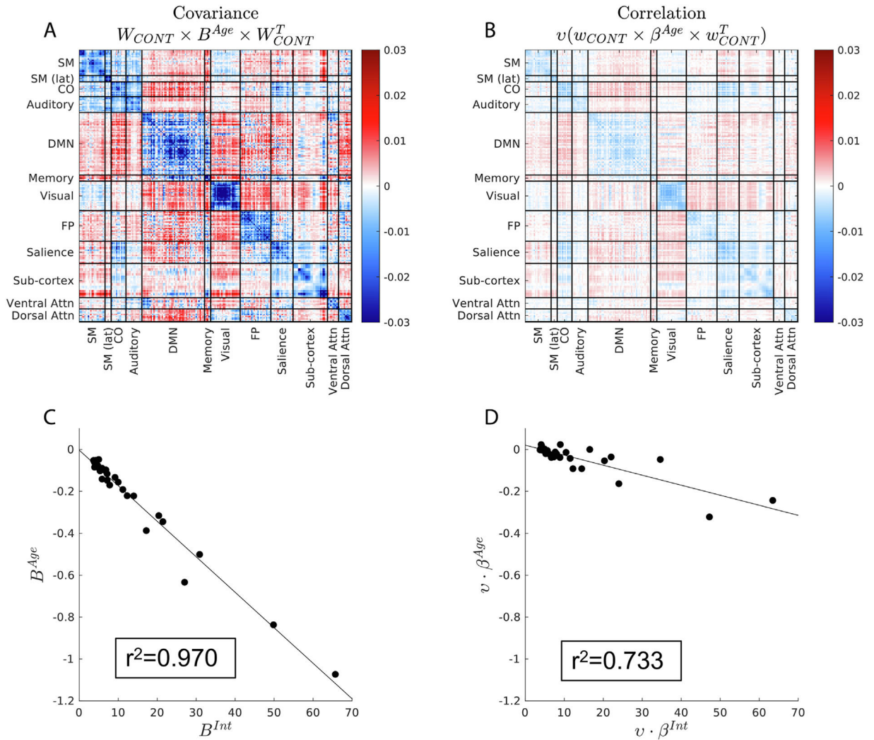
Fig. 5. Effect of age in the control participants. Panel A shows the effects of age on covariance FC, evaluated as \widehat{W}[\text{diag}B^{age}]\widehat{W}^T . Panel B shows the corresponding correlation FC result, evaluated as v_{CONT}\widehat{w}[\text{diag}\beta^{age}]\widehat{w}^T . The scales are identical. The effect of cohort has been removed by regression. Panel C shows B_j^{Age} plotted against B_j^{Int} , the intercept term, i.e., the value of covariance component j extrapolated to age 0. Note approximately uniform proportional effect of age across components ( r^2=0.970 ). The slope the fitted line indicates -1.69\% covariance component change per year relative to value at age 0. Panel D shows v_{CONT}\beta_j^{Age} plotted against v_{CONT}\beta_j^{Int} , i.e., correlation result parallel to panel C. The slope the fitted line is -0.48\% correlation component change per year relative to value at age 0. r^2 values (variance accounted for by the linear model) are included in insets in panels C and D for comparison to r^2 values reported in Fig. 8.
