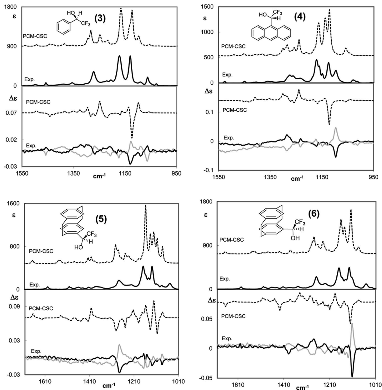
Fig. 3 Comparison of calculated VCD (lower part of each panel) and IR (top part of each panel) spectra of the (R) -enantiomers/diastereomers with the corresponding experimental spectra of the (R) and (S) enantiomers of four chiral aryltrifluorocarbinyloxy compounds, aryl = phenyl, 3 (top left), = anthryl, 4 (top right), and = [2.2]paracyclophan-4-yl, (R p ) - 5 and (S p ) - 5 (bottom left and right, respectively). Data from ref. 40. No scaling factor applied.
