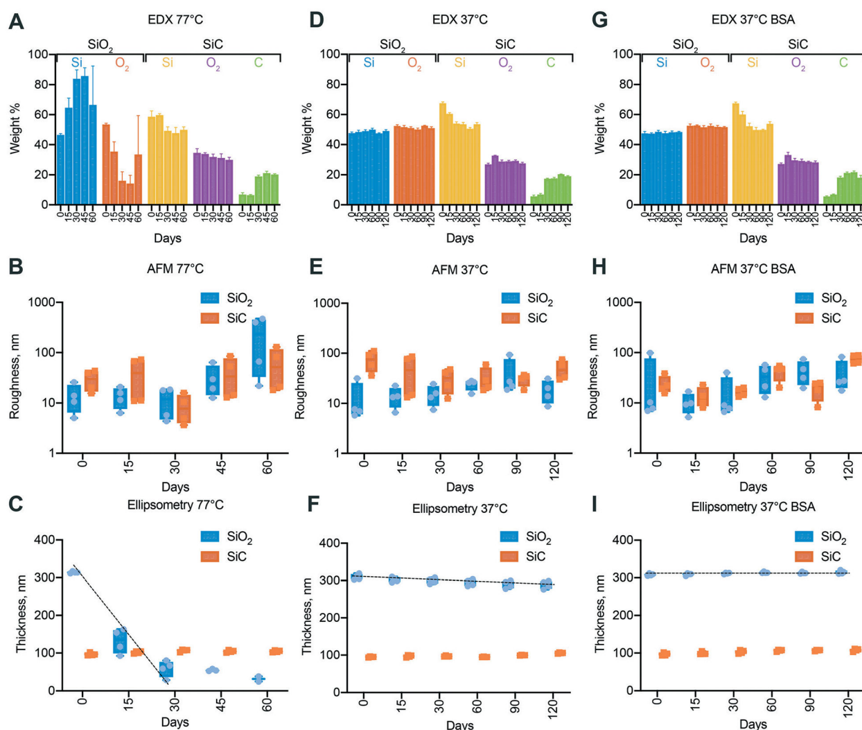
Fig. 3. Nanofluidic membrane degradation. Energy-dispersive X-ray spectroscopy (EDX) for membranes coated with \text{SiO}_2 versus \text{SiC} at 77 °C (A), 37 °C (D) and at 37 °C with BSA (G). Surface roughness calculated with atomic force microscopy (AFM) for membranes coated with \text{SiO}_2 versus \text{SiC} at 77 °C (B), 37 °C (E) and at 37 °C with BSA (H). Layer thicknesses fitted through ellipsometry data for membranes coated with \text{SiO}_2 versus \text{SiC} at 77 °C (C), 37 °C (F) and at 37 °C with BSA (I).
