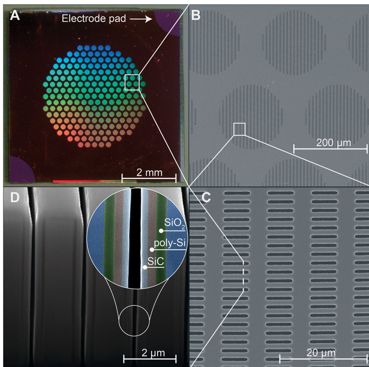
Fig. 2. Nanofluidic membrane. A) Picture of the nanofluidic membrane which measure 6\text{ mm} \times 6\text{ mm} with a total thickness of 400\text{ }\mu\text{m} . B) SEM image of the top face of the membrane (device layer) that shows the vertically etched nanochannels arranged in circles. C) SEM image of nanochannels array. D) FIB-SEM image of nanochannel cross-section which shows the vertical nanochannels and highlight the layer stack on the nanochannels walls. In order from the innermost (silicon, blue) to the outermost layer there is silicon dioxide ( \text{SiO}_2 , 175 nm, green), n-doped polycrystalline silicon (poly-Si, 121 nm, red) and silicon carbide (SiC, 64 nm, gray). The different layers in the FIB image are artificially colored for clarity.
