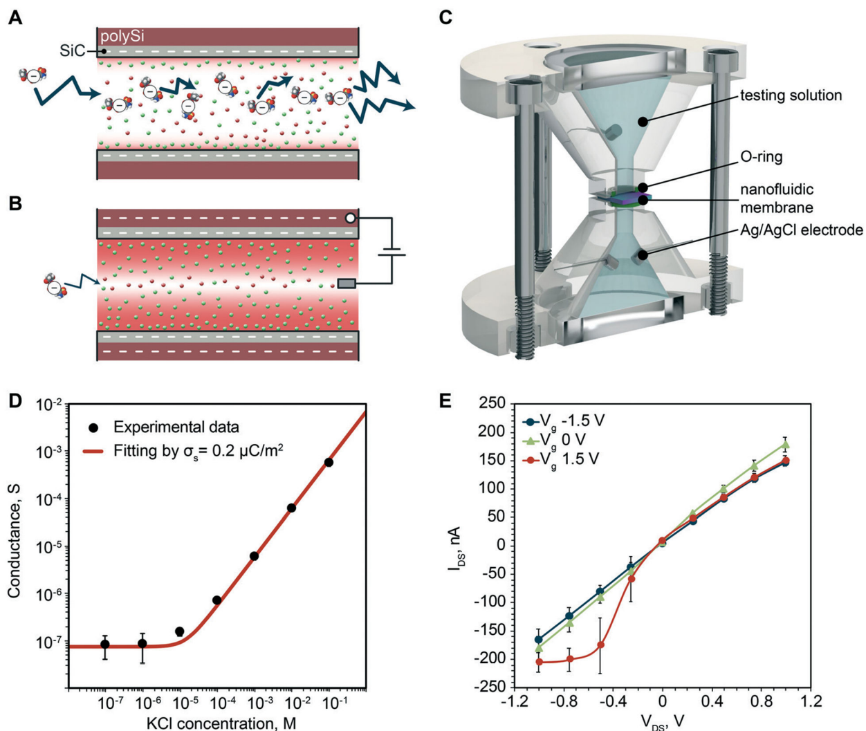
Fig. 5. Electrochemical characterization. A) Concentration driven diffusion of negatively charged molecule. B) Gated diffusion of negatively charged molecule. C) Rendering of ad hoc device for electrochemical measurements. D) Measured ionic conductance of the membrane. E) Current–voltage ( I – V ) curves for the membrane.
