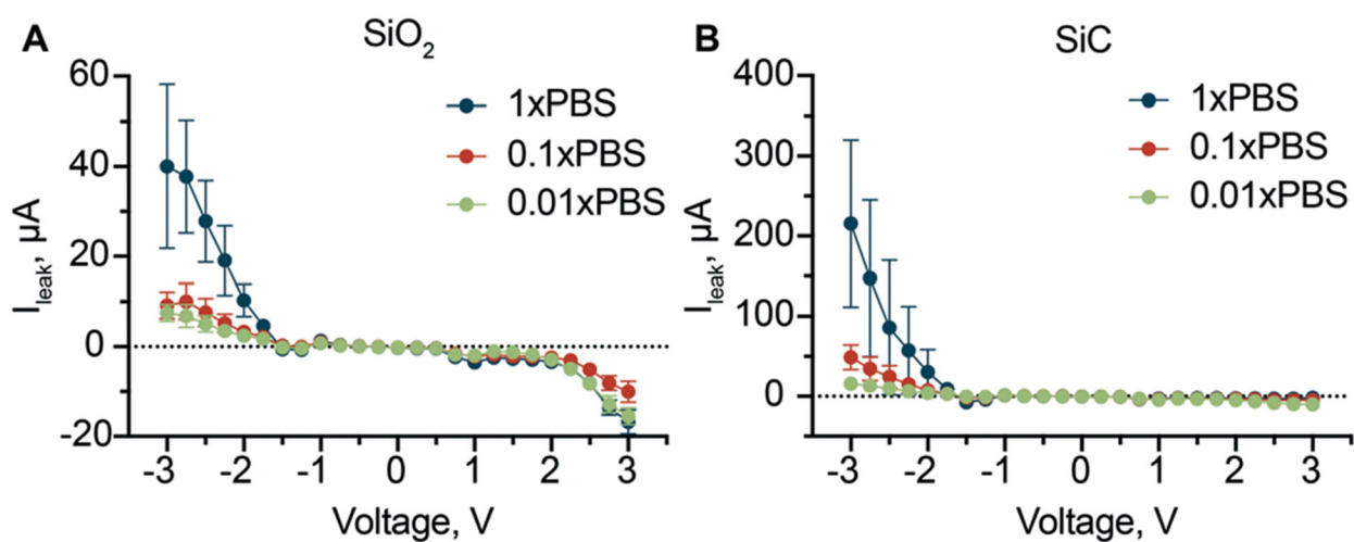
Fig. 4. Gate leakage current. Gate leakage current at different solution concentrations for \text{SiO}_2 dielectric layer (A) and \text{SiC} dielectric layer (B).
