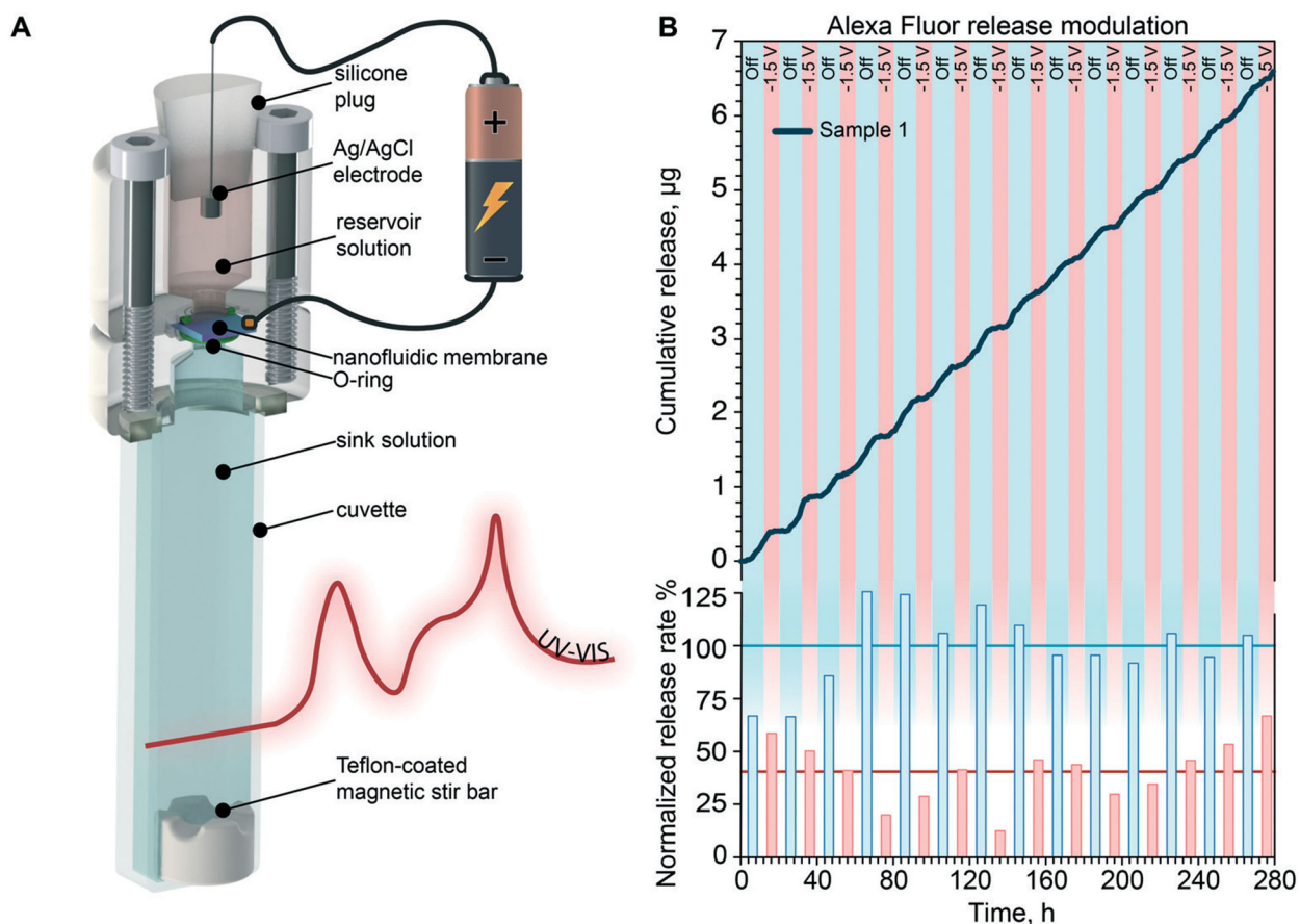
Fig. 6. Modulated release of Alexa Fluor 647. A) Rendering of custom device used for in vitro release rate modulation. B) In vitro cumulative release modulation of Alexa Fluor (top). Release rate for every phase, normalized to the average of the passive phases. Blue and red line represent the average of the passive and active ( -1.5\text{ V} ) phases respectively.
