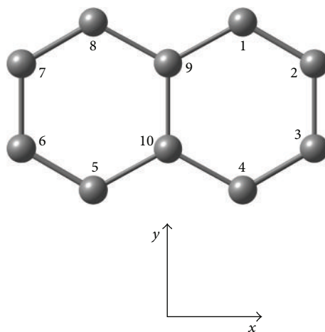
FIGURE 1: Coordinate system and atom numbering of dimethylnaphthalene (DMN) isomers.
