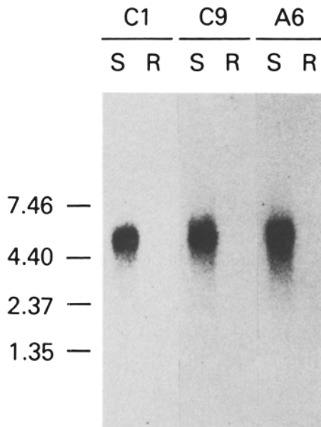
FIGURE 2. Northern blot of total RNA from WB C1, WB C9, and WB A6 probed with M2-1 and washed at 65^\circ\text{C} in 0.1\times\text{SSC} , 0.1\% SDS. In adjacent lanes are the 6E7S clones (S) and their 6E7R (R) antigenically variant progeny. Positions of RNA size markers (Bethesda Research Laboratories) are indicated on the left. The transcripts identified are \sim 5.4 kb.
