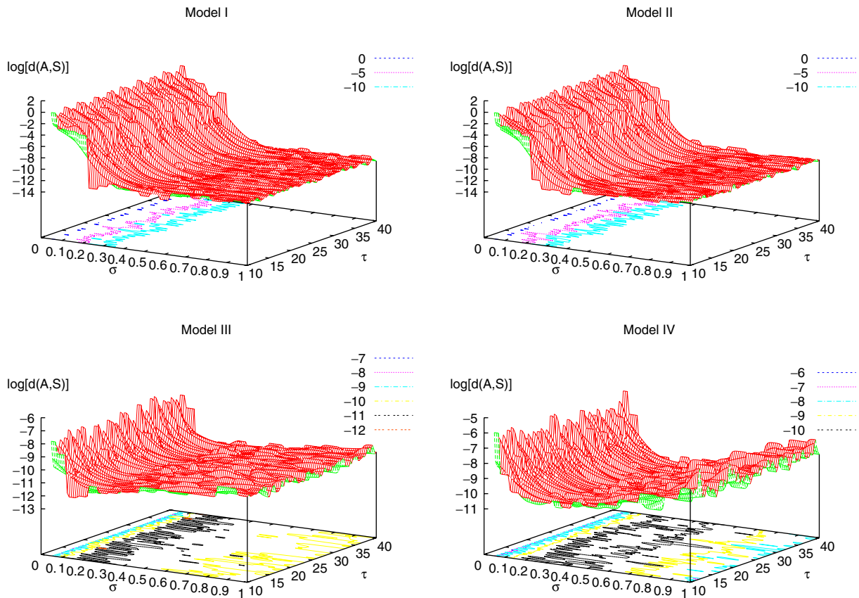
Figure 5 | Average value of \log[d(\Omega, S)] for the models I (top left)-II (top right)- III (bottom left)- IV (bottom right) with \sigma \in [0.01, 1] , \tau_L \in [10, 40] ms.
