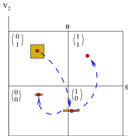
Figure 2 | Schematic representation, for two neurons, of the natural partition \mathcal{P} and the mapping discussed in the text. In this case, a firing state is a vector with components \omega = \begin{pmatrix} \omega_1 \\ \omega_2 \end{pmatrix} labeling the partition elements.
