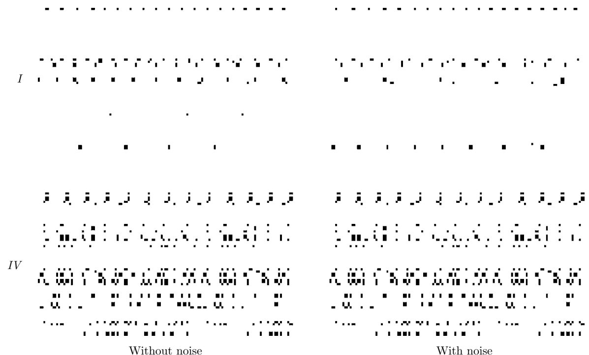
Figure 9 | Raster plots for models I (upper row) and IV (lower row), with \sigma = 10.00 and the same condition as in Figure 8. First column: model I and model without noise. Second column: same realization of synaptic weights and same initial conditions but with a small amount of noise in the external current. The noise is added to the membrane potential and its magnitude is very small ( 10^{-4} \times \theta ). One blob width is 1 msec.
