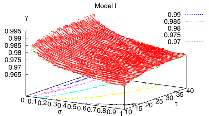
Figure 3 | Average value of \gamma for model I \sigma \in [0.01, 1] , \tau_L \in [10, 40] ms. The profile is very similar for other models.
