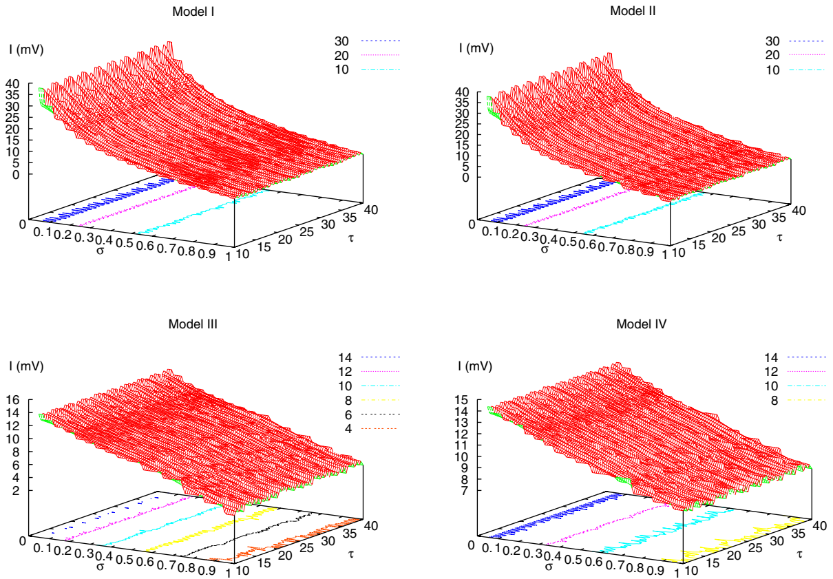
Figure 4 | Average current I for the models I (top left)-II (top right)- III (bottom left)- IV (bottom right) with \sigma \in [0.01, 1] , \tau_L \in [10, 40] ms.
