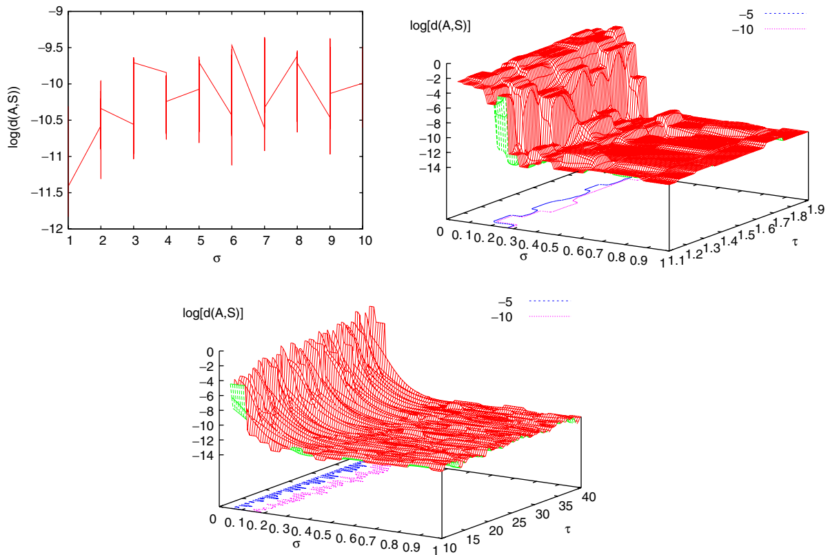
Figure 7 | Average value of \log[d(\Omega, S)] for the model I (left) \sigma \in [1, 10] , \tau_L \in [10, 40] ms. We present here a projection in the plane \sigma , \log[d(\Omega, S)] , and the vertical bars correspond to the variations with \tau_L . It allows us to verify the stability of the previous result for higher variability of the synaptic weights. (middle) \tau_L \in [1, 1, \dots, 2] ms below the usual 20 ms value, \sigma \in [1, 10] . Such range corresponds to cortical neurons in high-conductance state. It allows to check the behavior of d(\Omega, S) in this case. (right) Sampling period of 1 ms, in order to verify the robustness of the numerical results with respect to the sampling rate.
