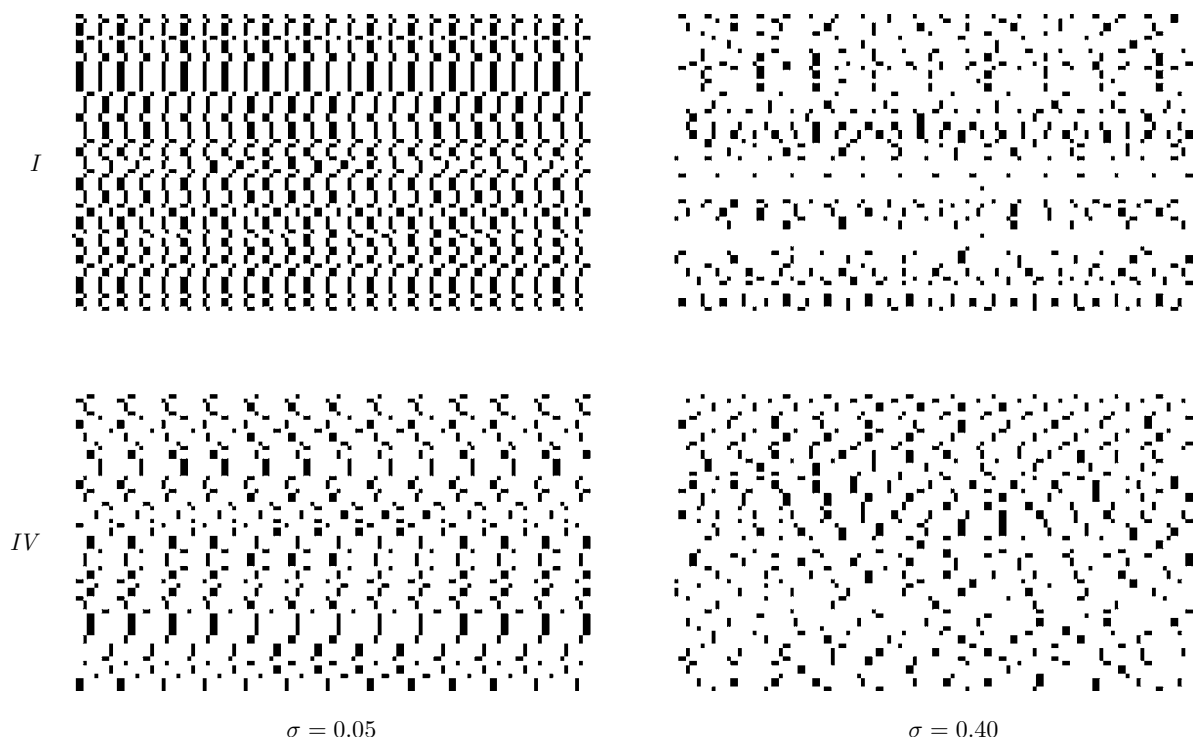
Figure 8 | Examples of raster plots for the conductance based model (Model I, top row) and the leaky integrate and fire model (Model IV, bottom row). A time window of 100 samples is shown in each case. The control parameter is \tau_L = 20 ms. As visible in Figure 5, \sigma = 0.05 corresponds to a small order dynamics where the periodic behavior is clearly visible, and \sigma = 0.40 to the “edge of chaos”. One blob width is 1 msec.
