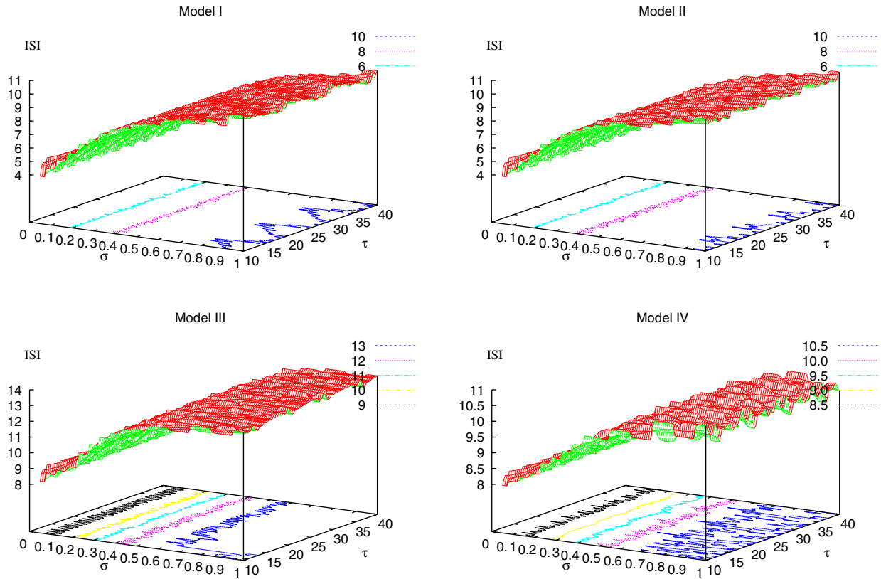
Figure 6 | Average value of the ISI for the models I (top left)-II (top right)- III (bottom left)- IV (bottom right), with \sigma \in [0.01, 1] , \tau_L \in [10, 40] ms.
