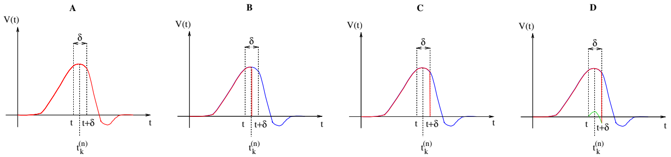
Figure 1 | (A) “Real spike” shape; the sampling window is represented at a scale corresponding to a “small” sampling rate to enhance the related bias. (B) Spike shape for an integrate and fire model with instantaneous reset, the real shape is in blue. (C) Spike shape when reset occurs at time t + \delta (Alternative I). (D) Spike shape with reset at time t + \delta plus addition of the integrate current (green curve) (Alternative II).
