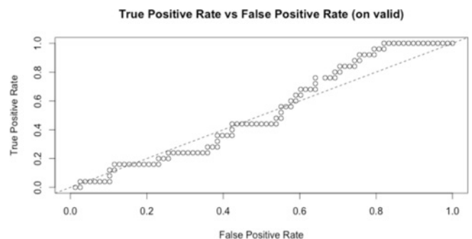
Figure 3 A typical receiver operating characteristic (ROC) curve for DL1 models derived from a fivefold cross-validation. The number of true 0s and true 1s in the data set used to train DL1 is balanced and thus the area under the ROC curve is quite poor despite the fact that this model is excellent at predicting true 1s. DL, deep learning paradigm.
