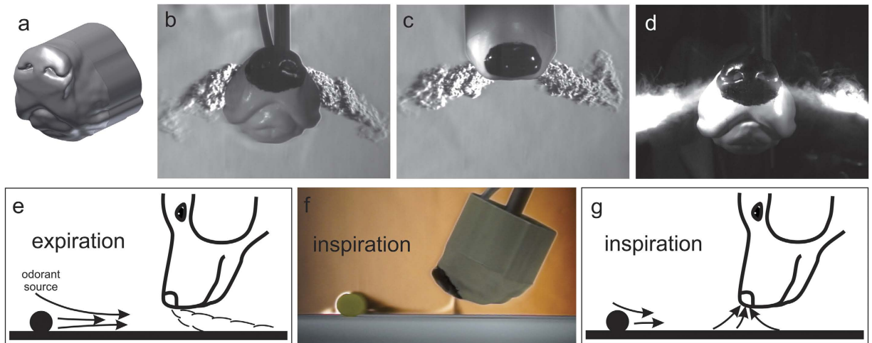
Figure 1. Jet-assisted fluid entrainment extends the aerodynamic reach of the canine nose during active sniffing. (a) Reconstructed model of the canine nose based on the model of Craven et al. 36,38,59 (2007, 2009, 2010) that includes the nasal vestibule, external nose, lower jaw, and about 10 cm of the snout. (b,c) Images extracted from high-speed schlieren videography flow visualization with helium illustrate the directionality of the expelled air jets from anterior (b) and dorsal (c) views. (D) Visualization of theatrical fog shows the ventral-laterally directed turbulent air jets exiting the naris during expiration. (e) During the expiratory phase of sniffing, turbulent air jets vectored ventrally and laterally entrain odorant vapor from tens of centimeters ahead of the nose that would otherwise be inaccessible to the dog. (f) Schlieren image of the 3D printed dog's nose during the inspiratory phase of sniffing showing acetone vapor be drawn into the nose from a source that is located approximately 10 cm away. (g) During the inspiratory phase of sniffing each nostril draws in air from all directions, including odorant-laden air that was drawn toward the nose during expiration. See Supplemental Information for video footage of these visualizations.
