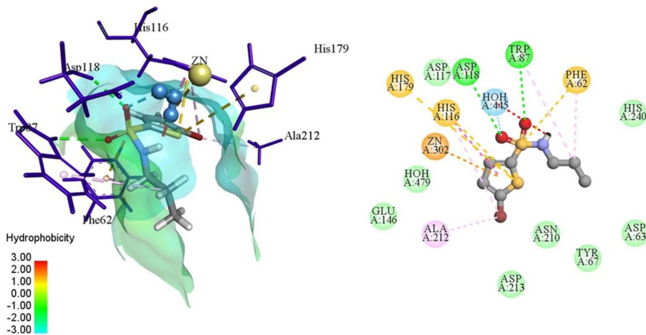
Figure 4 The left side of the image shows 3D interaction and the right side shows the 2D interaction of ligand (3b) with amino acid residues of the pocket. Interaction with zinc and water is clearly shown in the 2D demonstration.
