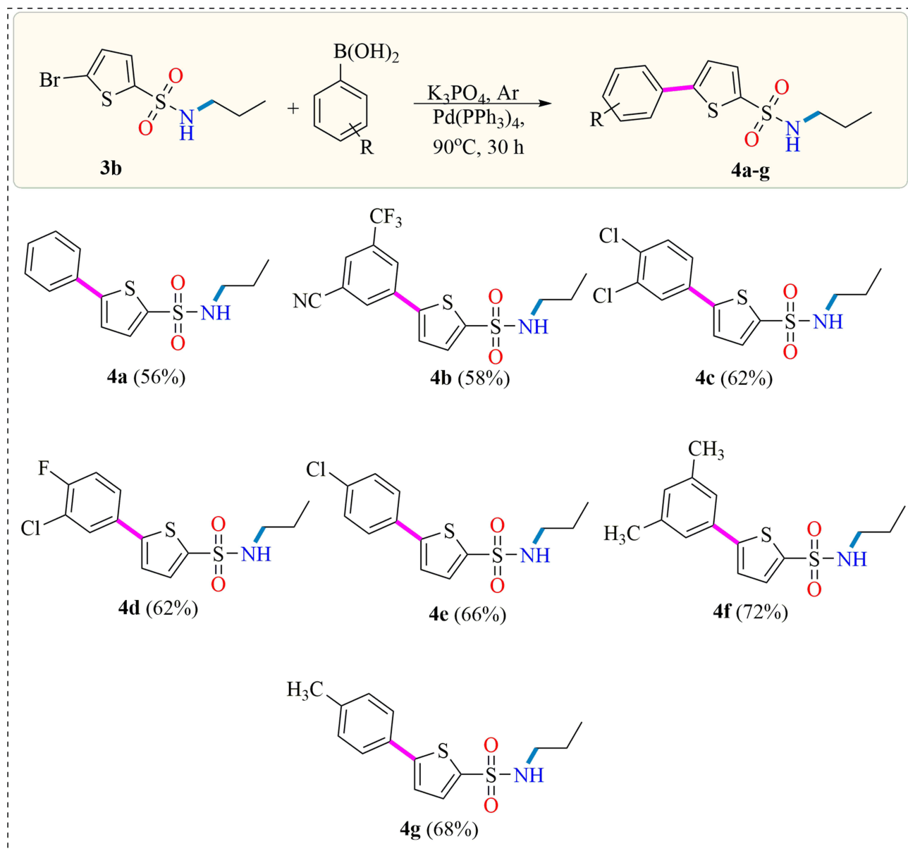
Figure 2 Arylation of 5-bromo-N-propylthiophene-2-sulfonamide.
