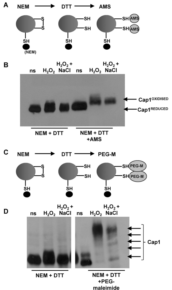
FIG 2 Cap1 oxidation following oxidative and combinatorial stresses. (A) Diagram showing the sequential NEM-DTT-AMS treatments employed to allow for the detection of disulfide bonds. (B) The oxidized forms generated following both oxidative and combinatorial stresses contain disulfide bonds. Cap1 mobility was monitored by nonreducing SDS-PAGE and Western blotting of proteins prepared from cells expressing Cap1-HM, under non-stress conditions (ns [Cap1 REDUCED ]) or following treatment with the indicated compounds. Samples were phosphatase treated prior to loading. The presence of disulfide bonds is indicated by the retarded mobility of Cap1 due to AMS binding to DTT-resolved disulfides (Cap1 OXIDISED ). (C) Diagram showing the sequential NEM-DTT-PEG-maleimide (PEG-M) treatments that allow for the detection of disulfide bonds. (D) Comparison of Cap1 oxidation before (ns) and following oxidative and combinatorial stresses by PEG-maleimide binding to DTT-resolved thiols. As in panel B, samples were phosphatase treated prior to loading. This shows that different oxidized forms of Cap1 are present following combinatorial stress, whereas a single form containing multiple disulfides is prevalent following oxidative stress.
