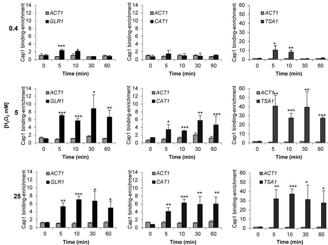
FIG 6 Quantification of Cap1 enrichment at the GLR1 , CAT1 , and TSA1 promoter targets. Cells expressing Cap1-MH (JC948) were treated with 0.4, 5, or 25 mM H_2O_2 for the indicated times and subjected to ChIP. The recovered DNA samples were analyzed by qPCR using primers specific for promoter regions within GLR1 , CAT1 , and TSA1 . Relative Cap1-MH enrichment values ( n -fold) are presented (mean \pm SD; n = 3 ). The following P values were considered: *, P \leq 0.05 ; **, P \leq 0.01 ; and ***, P \leq 0.001 .
