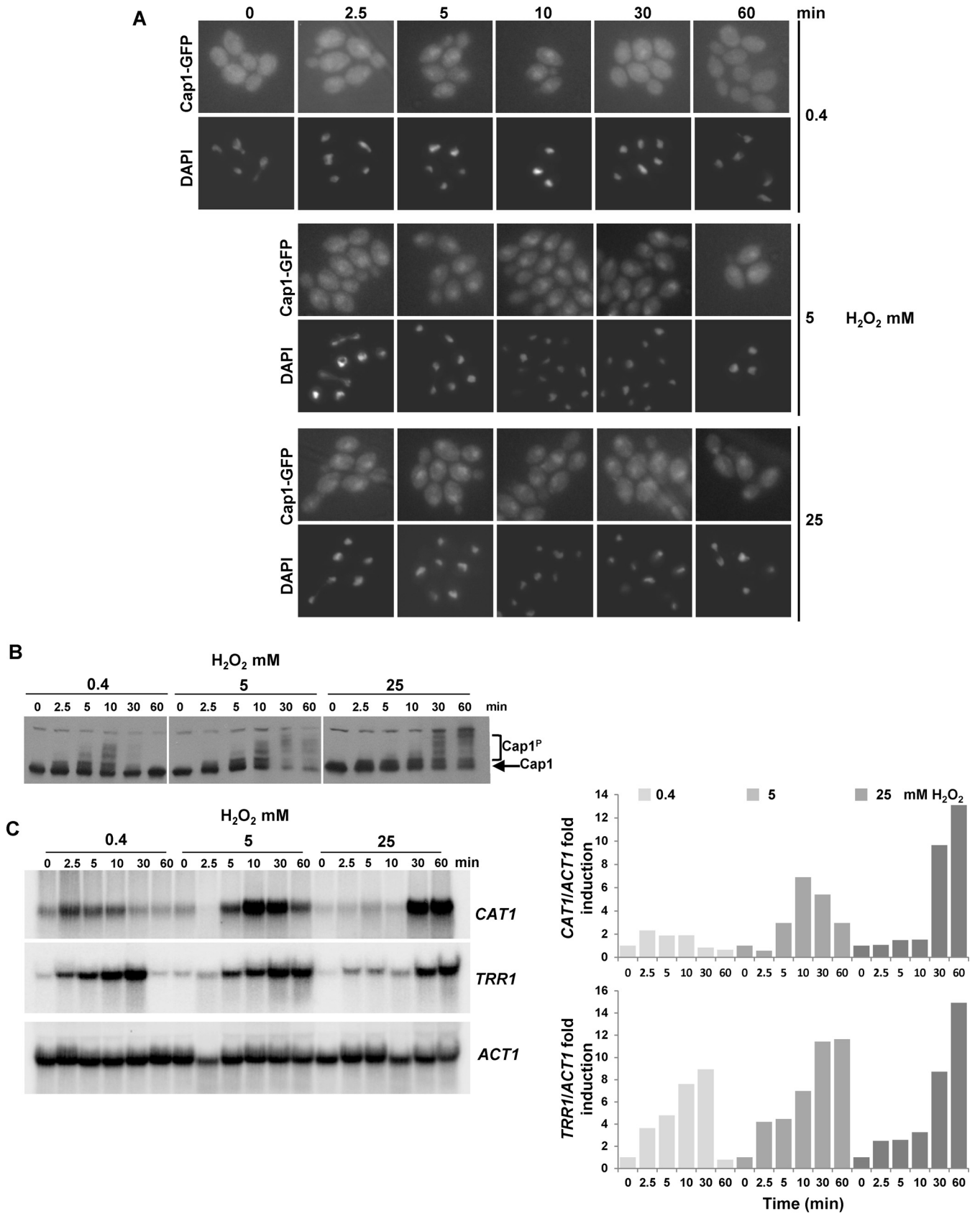
FIG 5 Cap1 rapidly accumulates in the nucleus in response to high levels of H 2 O 2 , but Cap1 phosphorylation and Cap1-dependent gene expression are delayed. (A) Cap1 localization was detected as described in the legend to Fig. 1B following treatment of Cap1-GFP cells with 0.4, 5, or 25 mM H 2 O 2 for the times indicated. (Continued)
