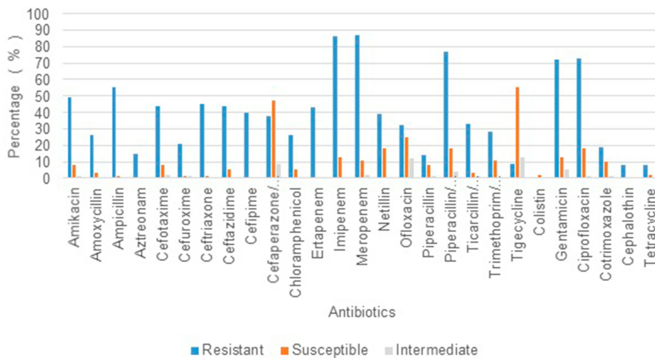
Figure 2 (N = 100): Percentage of isolates showing resistance to particular antibiotics.
