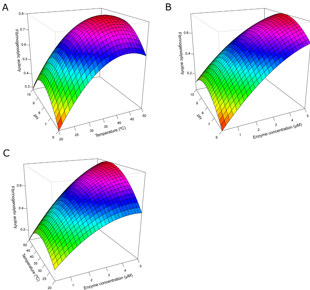
Fig. 3. Surfaces showing the response for two variables at a time. The variable not shown in each plot was kept at the stationary point. (A) Temperature ( ^{\circ}\text{C} ) vs pH, slice at enzyme concentration of 5\ \mu\text{M} ; (B) enzyme concentration ( \mu\text{M} ) vs pH, slice at 43.27\ ^{\circ}\text{C} ; (C) enzyme concentration ( \mu\text{M} ) vs temperature ( ^{\circ}\text{C} ), slice at pH 8.
