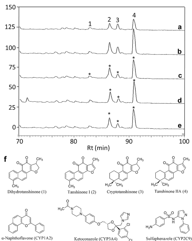
Fig. 2 Identification of specific ligands of CYP1A2, 3A4, and 2C9 in human liver microsomes (HLM) from Danshen ethanol extract (DEE) using ultrafiltration-high-performance liquid chromatography (HPLC) with competitive probes. (a) Danshen ethanol extract incubated without HLM (blank group); (b) Danshen ethanol extract incubated with HLM (experimental group); (c) Danshen ethanol extract incubated with HLM in which the active site of CYP1A2 was blocked with a competitive probe (control group); (d) Danshen ethanol extract incubated with HLM in which the active site of CYP3A4 was blocked with a competitive probe (control group); (e) Danshen ethanol extract incubated with HLM in which the active site of CYP2C9 was blocked with a competitive probe (control group); (f) structures of identified ligands from Danshen ethanol extract (DEE) and competitive probes. \alpha -Naphthoflavone, ketoconazole, and sulfaphenazole were used as competitive probes for CYP1A2, 3A4, and 2C9, respectively. Asterisk indicates the ligands identified using the present method. Compound 1 is dihydrotanshinone; compound 2 is tanshinone I; compound 3 is cryptotanshinone; compound 4 is tanshinone IIA.
