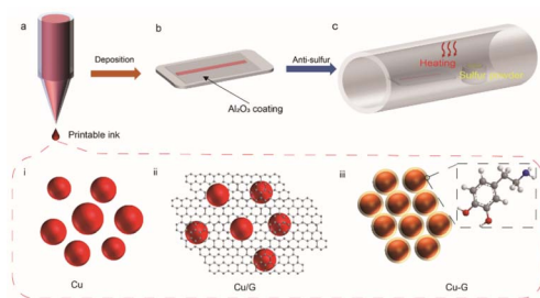
Fig. 1 Schematic of the Cu-based conductor for sulfur corrosion resistance. (a) Printing of the Cu-based conductors: Cu NPs (i), Cu/G (ii), and Cu-G (iii). (b) Cu-based conductor with a thin Al 2 O 3 layer coating. (c) Schematic of in situ measurement under a sulfurous atmosphere at different temperatures.
