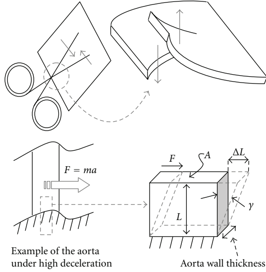
FIGURE 5: Shear stress.
