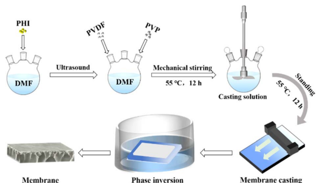
Fig. 1 Synthetic diagram of PHI/PVDF membranes.
