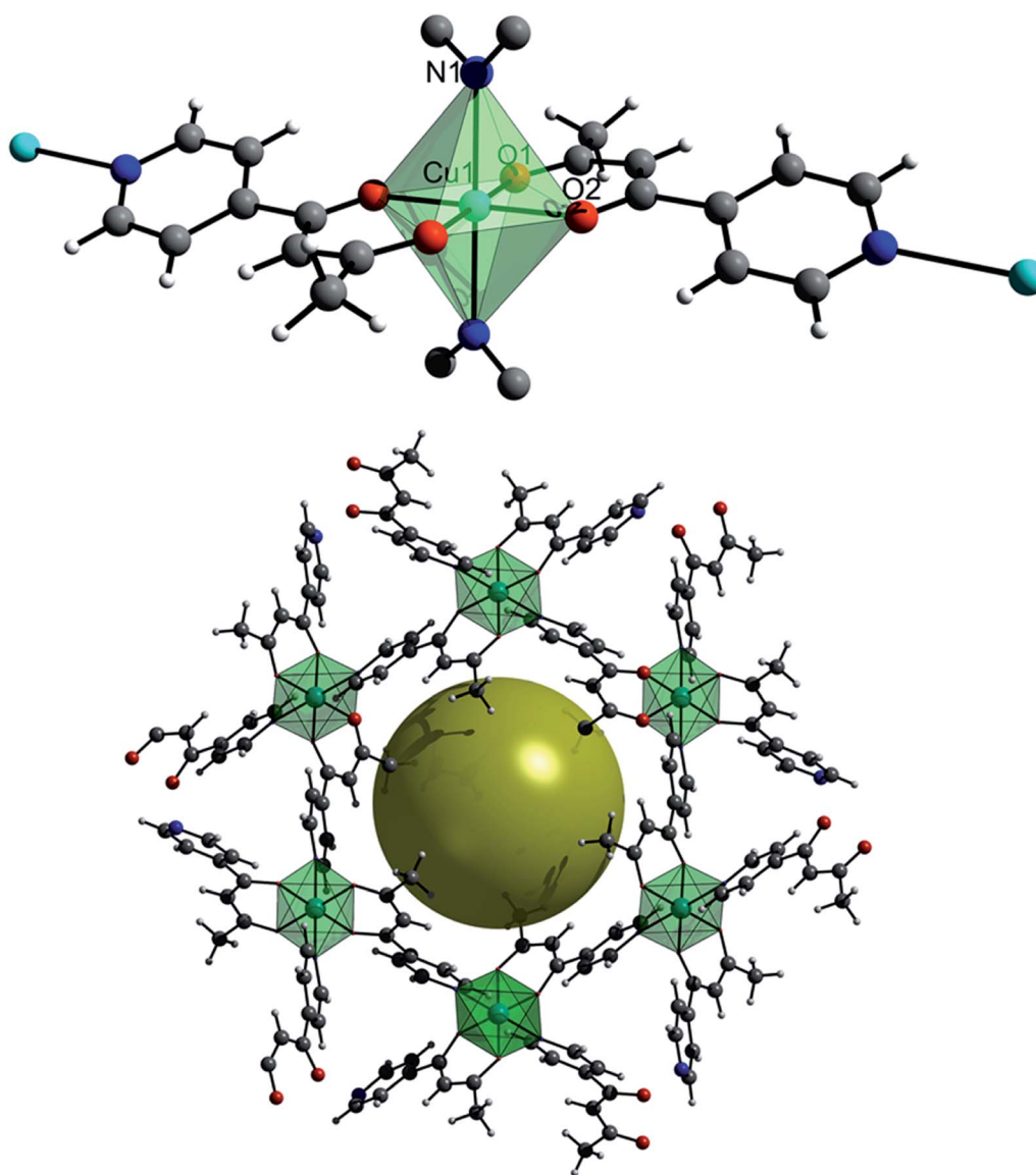
Fig. 1 Ball and stick model showing the coordination environment around the \text{Cu}^{2+} ion in CuPyr-I, and 3D-pore structure as viewed along the c -axis direction. The yellow sphere represents the available pore-space. Colour scheme is red: oxygen, blue: nitrogen, black: carbon, white: hydrogen and cyan: copper. The \text{Cu}^{2+} octahedron is illustrated in green.
