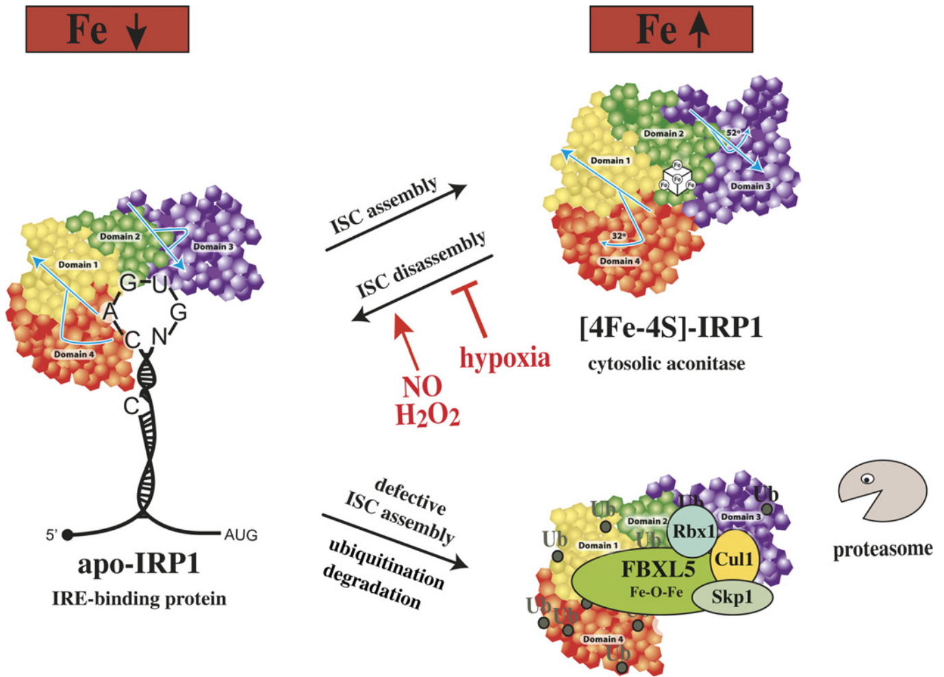
Figure 6 Under physiological conditions, IRP1 is regulated by a reversible ISC switch
