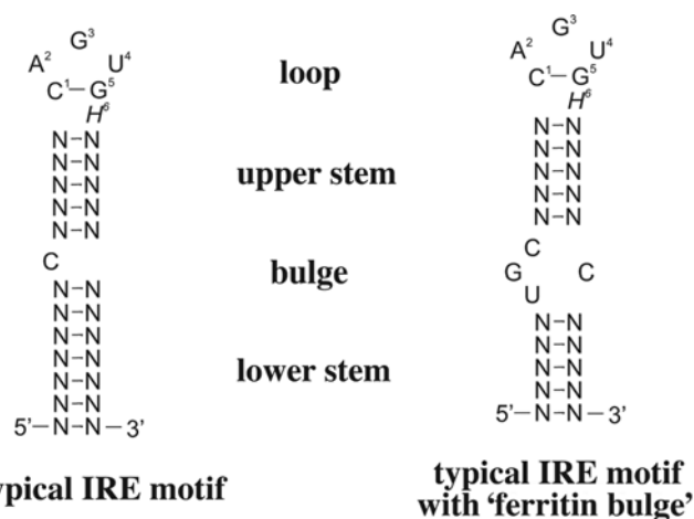
Figure 3 Typical IRE motif
