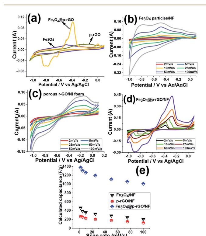
Fig. 10 (a) Comparison of the capacitive behavior of the fabricated NF electrodes at the scan rate of 5 \text{ mV s}^{-1} , (b–d) CVs of \text{Fe}_3\text{O}_4 /NF, rGO/NF and \text{Fe}_3\text{O}_4 @p-rGO/NF at the scan rates of 2–100 \text{mV s}^{-1} , (e) the calculated capacitances values vs. scan rate for the fabricated electrodes.
