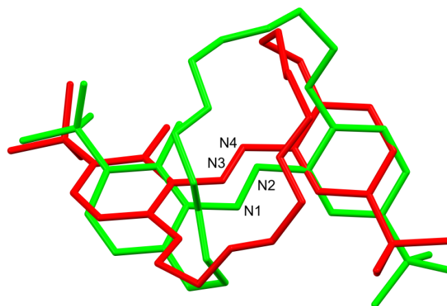
Figure 4. Comparison of the two symmetry-independent molecules of t -Bu-19- o -OH. Note the molecules are not just mutual mirror reflections since the ether linker has significantly different conformation. Colours by symmetry equivalence. The green molecule contains the N1-N2 group, and the red one, containing N3-N4, is inverted, and the best overlap of the molecules is presented (RMSD 1.7196 Å and maximum distance of equivalent atoms 4.023 Å, generated by Mercury 2021.2.0 program). Conformations of ether chains are visibly different.
