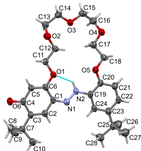
Figure 5. Molecular view of t -Bu-19- p -OH showing atom labelling scheme in one molecule, arbitrarily selected from the two symmetry-independent molecules in the structure. Intramolecular hydrogen bonding is drawn as the dashed cyan line. Displacement ellipsoids are drawn at a 50% probability level. Selected bond lengths (Å) and angles (°): N1–N2 1.315(6), N1–C1 1.325(7), N2–C19 1.413(7), C4–O6 1.242(6), C6–O1 1.360(6), C11–O1 1.439(6), C12–O2 1.437(6), C13–O2 1.407(7); valence angles: N2–N1–C1 122.4(4), N1–N2–C19 117.8(4), C6–O1–C11 115.6(4), C12–O2–C13 115.9(5), C14–O3–C15 112.1(4), C16–O4–C17 113.9(4), C18–O5–C20 117.3(4); torsions O1–C6–C1–N1 1.5(9), N2–N1–C1–C6 1.2(9), O5–C20–C19–N2 1.8(8). Torsions in the linker ether: (starting from C6–O1–C11–C12) –ap, –ap, –ac, –sc, +sc, +ap, –ap, –sc, +sc, +ap, +ap and +ap (C17–C18–O5–C20).
