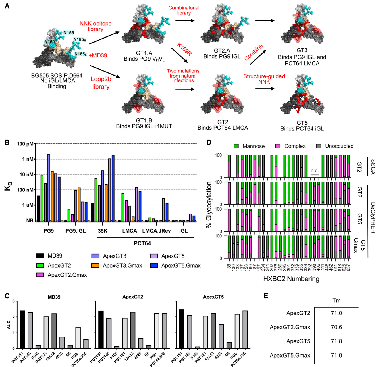
Figure 4. V2-apex germline-targeting immunogen design produces ApexGT trimers as candidate immunogens to prime PCT64 and PG9/16 responses
