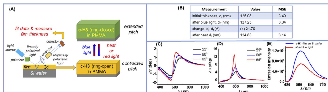
Fig. 5 (A) Schematic representation of spectroscopic ellipsometry (SE) measurement of a thin film of c-H3 in the PMMA matrix on Si wafer. (B) Thickness changes of a thin film of c-H3 in the PMMA matrix upon blue light irradiation (blue LED, 5.10 mW cm -2 ) and heating (80 °C); MSE = mean squared error of the fitting model applied to fit the data. See ESI† for details. (C) \delta\Psi/\Delta and (D) \delta\Delta/\Delta spectroscopic ellipsometry spectral difference of the film before and after the blue light irradiation, where \delta\Psi/\Delta = \Psi/\Delta before irradiation, -\Psi/\Delta after irradiation, and \Psi and \Delta are the ellipsometric parameters. (E) Emission spectral changes of a thin film of c-H3 (in PMMA) on Si wafer upon blue light (5.10 mW cm -2 ) irradiation (for 2 min).
