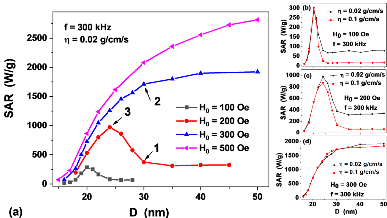
Figure 1. (a) SAR of a dilute assembly of magnetic nanoparticles depending on the particle diameter for different ac magnetic field amplitudes H_0 at the liquid viscosity \eta = 0.02 g/(cm s). (b–d) dependence of SAR on the liquid viscosity for various ac magnetic field amplitudes. Similar results were obtained also in Ref. 32 for other values of magnetic parameters.
