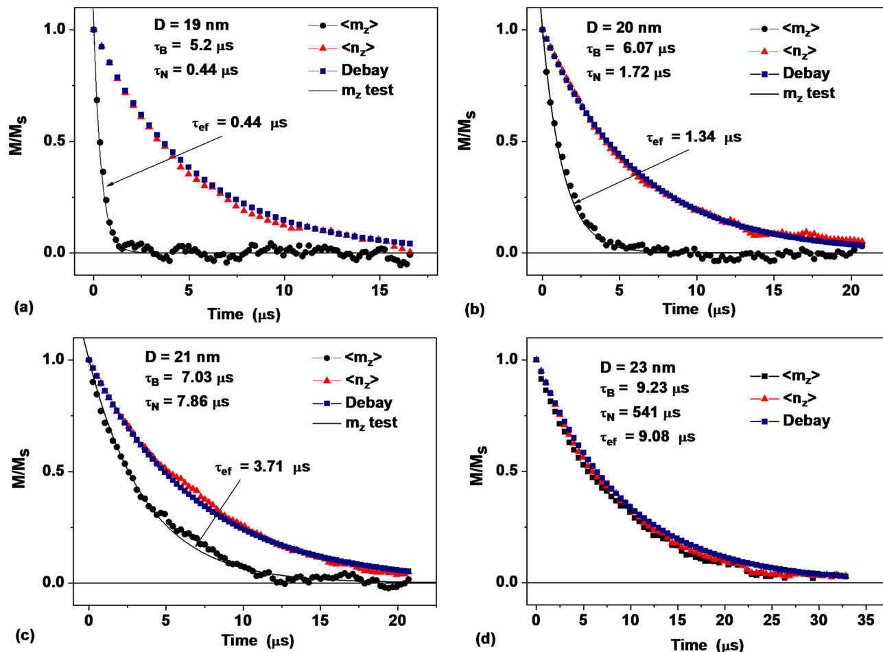
Figure 3. Relaxation curves of dilute assemblies of magnetic nanoparticles in a liquid with viscosity \eta = 0.02 g/(cm s) at a temperature T = 300 K for particles of different diameters: (a) D = 19 nm, (b) D = 20 nm, (c) D = 21 nm and (d) D = 23 nm. Circular and triangular dots show the time dependence of the projections \langle m_z(t) \rangle and \langle n_z(t) \rangle , respectively. The square dots show the Debye orientation relaxation process for nonmagnetic nanoparticles with the corresponding relaxation time \tau_B . The solid curves show the exponential approximation of the \langle m_z(t) \rangle dependence with the corresponding effective relaxation time \tau_{\text{ef}} Eq. (2).
