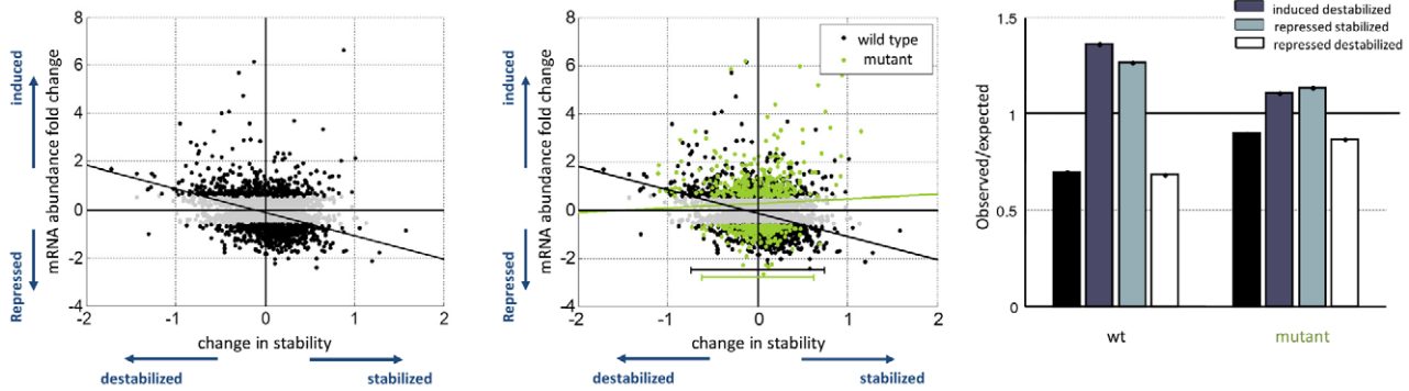
Figure 2. Reduced coupling in Rpb6 mutant strain. The change in mRNA stability relative to the reference state ( \log_2(I_{1/2\text{oxidative}}/I_{1/2\text{reference}}) ) is plotted against the maximal fold change, defined as the maximal change in mRNA abundance for each gene across the time course. (A) Shows the wild type strain where black dots marks genes which respond to the stress. A negative correlation by which induced genes are destabilized is illustrated by the plotted least square line ( R = -0.23 , -\log_{10}(\text{p-value}) > 58 ). Fitted line y = -0.97x - 0.12 with (-1.14, -0.7947) and (-0.1875, -0.05864) 95% confidence interval for each parameter. (B) The mutant measurements are plotted on top of the wild type. The negative correlation observed in the wild type, reflected by the black least straight line, is almost completely eliminated, displayed in the green least square line ( R = -0.06 , -\log_{10}(\text{p-value}) < 6 ). Fitted line y = 0.1852x + 0.27 with (-0.1723, 0.5426) and (0.1596, 0.3805) confidence interval for each parameter. Also the width of the distribution across the x-axis is slightly narrower for the mutant strain an indication for reduced ability to modulate mRNA stability. (C) Fold enrichment for the change in stability in induced and repressed genes. The number of observed stabilized and destabilized genes within both induced and repressed groups of genes divided by the expected number, assuming no correlation. Expected number is calculated as the percentage of stabilized/destabilized genes in the genome times the induced/repressed group size. doi:10.1371/journal.pgen.1002273.g002
