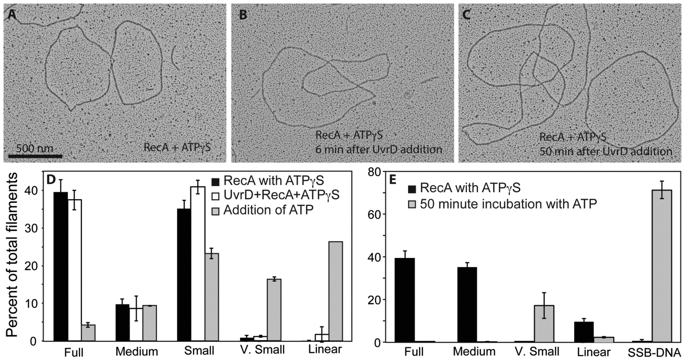
Figure 8. ATP hydrolysis by UvrD is required for dismantling RecA filaments. (A) RecA filaments formed on circular ssDNA after a 10 min incubation with 1 mM ATP γ S. Two full filaments and a very small filament, as well as SSB-coated DNA are present in this image. (B) RecA filaments formed as in (A), after a six-minute incubation with UvrD. (C) RecA filaments formed as in (A) after 50 min incubation with UvrD. No decrease in filamentation can be observed. (D) If 3 mM ATP is added with the UvrD helicase, significant disassembly of the RecA filaments is seen after 6 min. Molecules are quantified with RecA and ATP γ S alone ( n = 1027 molecules counted and scored), after addition of UvrD ( n = 1187 molecules counted and scored) and after further addition of ATP ( n = 1060 molecules counted and scored). (E) Experiment as in panel D, but with less ATP γ S (30 \mu M) added to form the RecA filaments, addition of UvrD, and filaments examined 50 min after further addition of 3 mM ATP. Molecules counted and scored ( n = 573 prior to and ( n = 581 at 50 min after addition of ATP).
