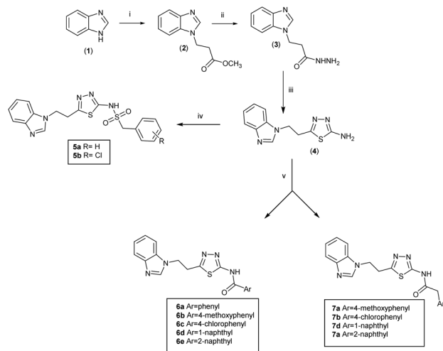
Scheme 1 Preparation of series 1 and 2. Reagents and conditions (i) K_2CO_3 , 18-crown-6, methyl 3-bromopropionate, DMF, 60 °C, o/n (ii) NH_2NH_2 , EtOH, r. t. o/n (iii) TMSNCS, ^iPrOH , H_2SO_4 , NH_4OH , reflux o/n (iv) R -appropriate phenylmethanesulfonyl chloride, DMAP, pyridine, CH_2Cl_2 , r. t. o/n (v) aryl carboxylic acid, TBTU, HOBT, DMF, DIPEA, r. t. o/n.
