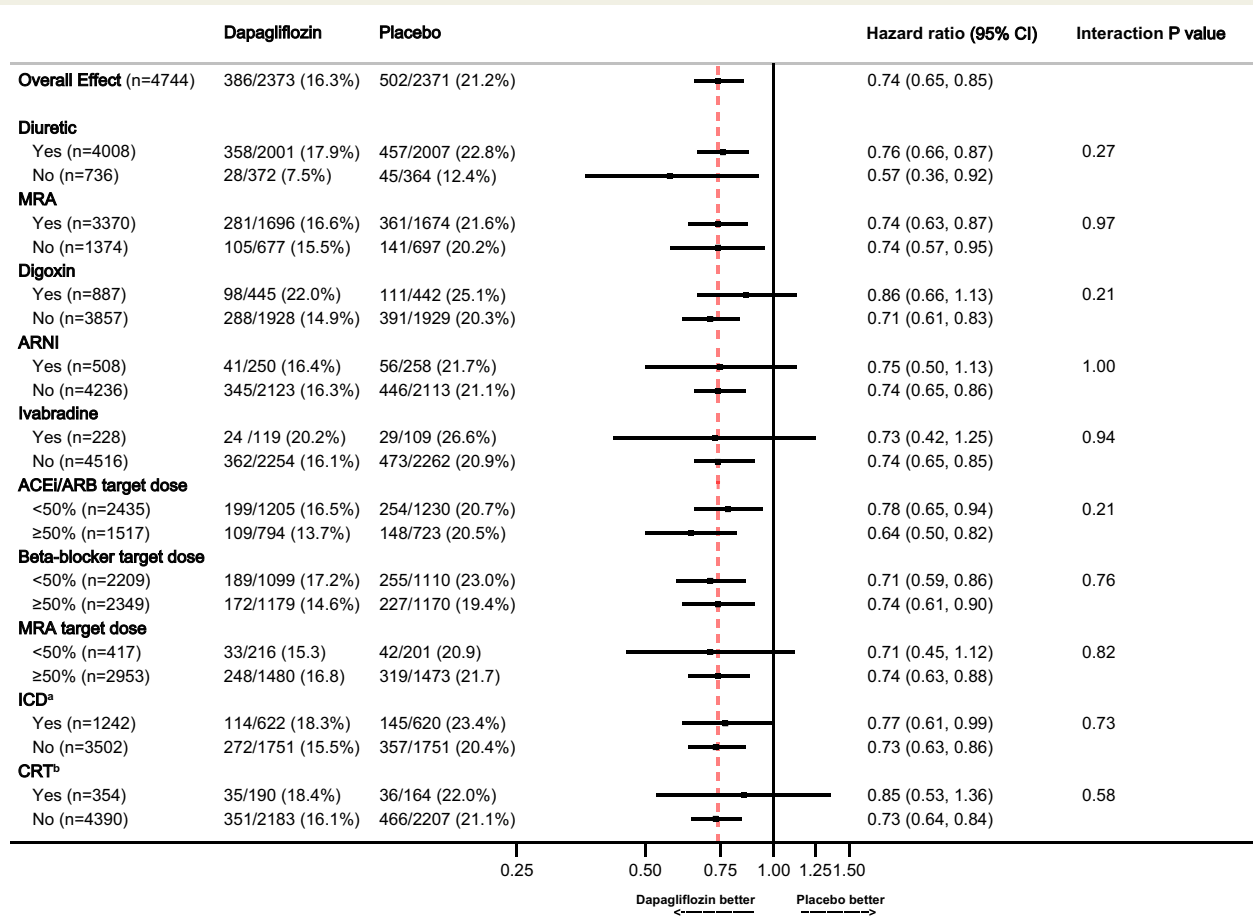
Figure 1 Effect of dapagliflozin compared to placebo on the primary composite outcome by background heart failure therapy. The primary outcome was a composite of worsening heart failure (hospitalization or an urgent visit resulting in intravenous therapy for heart failure) or death from cardiovascular causes. Hazard ratios and 95% confidence intervals were estimated with the use of Cox regression models, stratified according to diabetes status, with a history of hospitalization for heart failure, and treatment-group assignment as explanatory variables. ACEi, angiotensin-converting enzyme inhibitor; ARB, angiotensin receptor blocker; ARNI, angiotensin receptor neprilysin inhibitor; CI, confidence interval; CRT, cardiac resynchronization therapy; ICD, implantable cardioverter-defibrillator; MRA, mineralocorticoid receptor antagonist. a ICD or cardiac resynchronization therapy with defibrillator. b Cardiac resynchronization therapy with or without a defibrillator.
