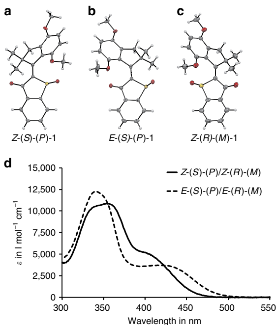
Figure 2 | Molecular structure and absorption characteristics of motor 1. (a) Crystal structure of racemic Z -( S )-(P)/ Z -( R )-(M) isomers, only the Z -( S )-(P) isomer is shown (CCDC 1061969). (b) Crystal structure of racemic E -( S )-(P)/ E -( R )-(M) isomers, only the E -( S )-(P) isomer is shown (CCDC 1061970). (c) Crystal structure of enantiomerically pure Z -( R )-(M) isomer (CCDC 1406625). (d) Extinction coefficients of the Z -( S )-(P)/ Z -( R )-(M) isomers (—) and the E -( S )-(P)/ E -( R )-(M) isomers (---) in \text{CH}_2\text{Cl}_2 .
