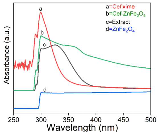
Fig. 3 UV-visible spectroscopy analysis of plant extract, cefixime, franklinite ( \text{ZnFe}_2\text{O}_4 ) and cefixime-loaded franklinite (Cef-ZnFe 2 O 4 ).
