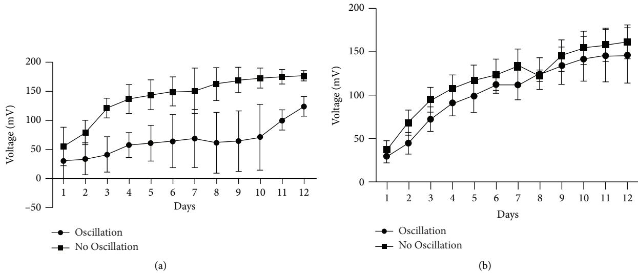
FIGURE 6: The effect of oscillating vs nonoscillating conditions on MFC voltage (mV ± SD) output by H. salinarum at 37°C using either (a) 5 cm 2 or (b) 10 cm 2 size platinum carbon cloth electrodes. Nonoscillating conditions significantly ( p < 0.0001 ) affected voltage with a 5 cm 2 electrode size, while there was no change ( p = 0.3709 ) with 10 cm 2 sized electrodes as per an unpaired T -test with welch correction.
