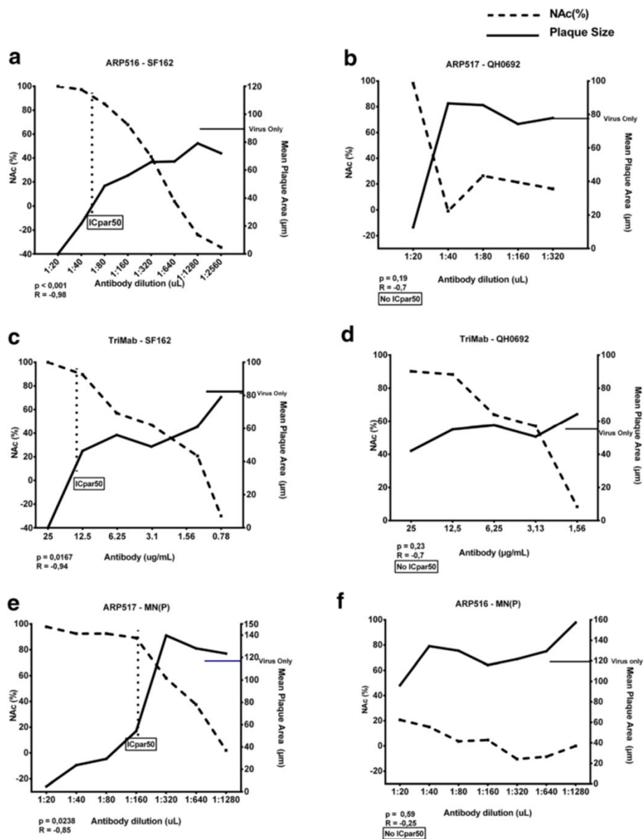
Figure 8 Relationship between neutralization and plaque area. —, mean plaque area (µm, y axis on the right) indicated with a solid line; - - - - - , neutralization (NAC%, y axis on the left) indicated with a broken line in each panel and ICpar50 values are indicated with vertical dotted lines in panel a , b and c . The plaque area without addition of inhibitory reagent (virus only) is indicated by a horizontal line on the y axis on the right. Virus-plasma combinations: (a) ARP516-SF162; (b) ARP517-QH0692; (c) TriMab-SF162; (d) TriMab-QH0692; (e) ARP517-MN(P); (f) ARP516-MN(P). R and p values are given for the correlation of neutralization and plaque area according to Spearman rank.
