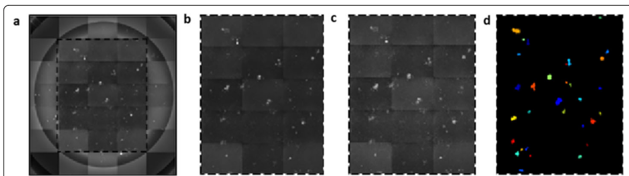
Figure 1 The APR assay pipeline tiles the inner 15 images from each well (a) into a mosaic (b). The pipeline includes algorithms for illumination correction (c) and plaque identification (d). The colors labeling the plaques are used for illustrative purposes and chosen arbitrarily by the program.
