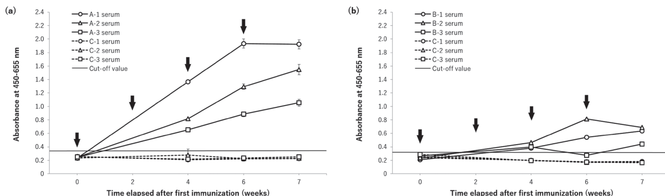
Fig. 1. Antibody titers (absorbance at 450–655 nm; mean \pm SD) in mongoose sera following immunization with peptide A (a) and peptide B (b). Horizontal lines mean the cut-off value calculated from each control on same microplate: cut-off value=mean antibody titer of control + 3 SD. Arrows indicate the times of immunization.
