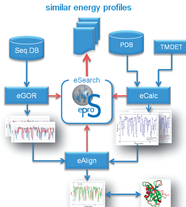
Figure 5. The eProS toolbox affords several, interconnected methods for accessing and working with the eProS database. Besides energy profile data access and calculation (eCalc), methods for predicting (eGOR) and aligning (eAlign) energy profiles have been implemented. These techniques can be used to derive or retrieve energy data that can be queried for at the eProS database (eSearch). Identified significantly similar energy profiles can be further investigated. Provided annotations and detected similarities can aid in understanding the dynamics and functional aspects of the protein of interest.
