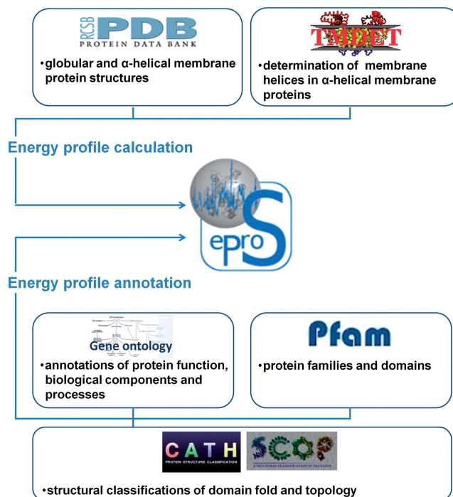
Figure 2. The eProS database integrates data from the PDB (12) and TMDET (energy profile calculation) as well as the Gene Ontology database (13), CATH (14), SCOP (15) and Pfam (16) (energy profile annotation). Energetic discrepancies and similarities between proteins can be investigated by the eProS toolbox. The energy profile annotations provided by the data integration can broaden the understanding of the relationships between energetic, functional and structural properties. Furthermore, the advanced reverse annotation lookup can be a valuable method to identify functional- and structural-related proteins and study their energetic similarities.
