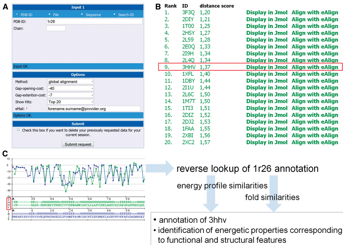
Figure 4. eSearch is a tool that provides eProS-wide searching for similar protein energy profiles. It can be queried (A) by specifying an energy profile by its PDB ID, by uploading a structure from which the corresponding energy profile is subsequently computed or by specifying a sequence. In the last case, an energy profile prediction algorithm (eGOR) is applied. Because of long computing times, the user has to enter a valid e-mail address. Access to previous search results is provided by direct-links and session ids sent by e-mail. eSearch results are given as lists that are ranked according to derived distance scores (dScores) (B). In general, the dScore reports the significance of the resulting energy profile alignment and, thus, energy profile similarity (see the Supplementary Data for further details). In this example, the Trypanosoma brucei brucei thioredoxin has been queried, leading to a list of various energetically similar protein structures (hits). For the ninth hit (PDB ID 3hhv), no GO-term annotation is given. With respect to the energy profile alignment (C) and similarities obtained from energy profile analyses of further hits and entries retrieved by reverse annotation lookup, functional and structural energetic properties can be detected that are common in all identified energy profiles, including 3hhv. From this, GO-term annotations for 3hhv can be proposed.
