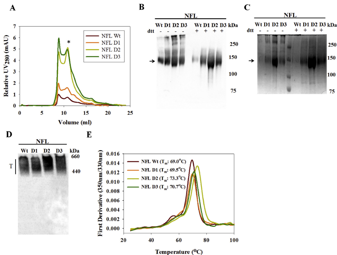
Fig. 2. Biophysical characterization of NFL designs. A: Relative UV 280 chromatograms of lentil lectin purified designs subjected to SEC purification on an S200 column. * Trimer fraction peak ~10.8 ml. B, C: Reducing (+) and non-reducing (-) SDS-PAGE western and SDS-PAGE Coomassie brilliant blue stained gels respectively. Arrow indicating the size of the monomeric band resulting from denaturation (~140 kDa). D: Blue Native PAGE western of the SEC purified trimer. E: nanoDSF thermal melt of the SEC purified trimers.
