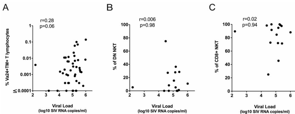
Figure 9. Relationship between plasma SIV RNA and NKT lymphocytes. (A) Correlation between plasma SIV RNA and peripheral blood frequency of V\alpha 24^+CD1d^+ TM^+ NKT lymphocytes in 43 SIV-infected sooty mangabeys. (B) Percentage of DN NKT lymphocytes and (C) percentage of CD8^+ NKT lymphocytes correlated with plasma SIV RNA in 15 SIV-infected sooty mangabeys. 'r' denotes correlation coefficient values determined by the Pearson correlation test. doi:10.1371/journal.pone.0009787.g009
