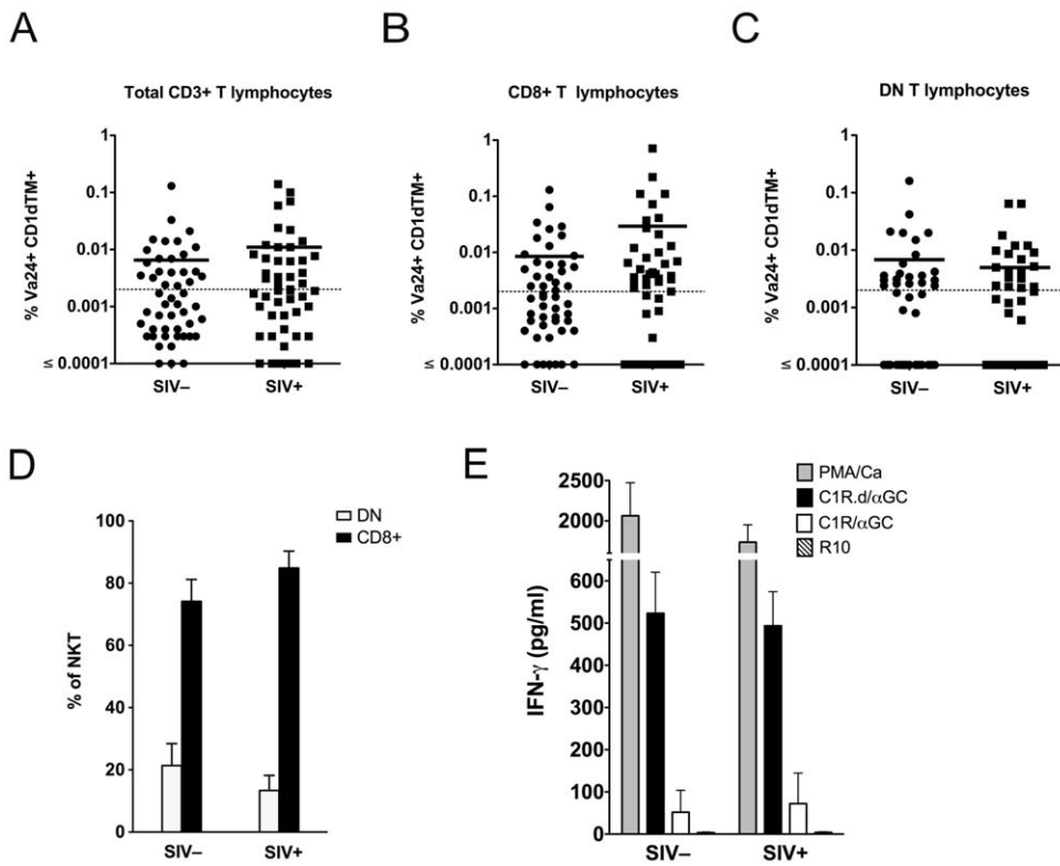
Figure 8. NKT lymphocytes are not depleted in SIV-infected sooty mangabeys. Frequency of peripheral blood V\alpha 24^+CD1d^+ TM^+ NKT lymphocytes in 50 SIV-negative and 50 SIV-infected sooty mangabeys as a percentage of (A) total circulating T lymphocytes, (B) circulating CD8^+ T lymphocytes, and (C) circulating DN T lymphocytes. Horizontal bar denotes mean. D) Percentage of CD8^+ and DN T lymphocyte subsets in peripheral blood NKT lymphocytes in SIV- and SIV+ sooty mangabeys. E) IFN-\gamma ELISA on 24-hour culture supernatants of ex vivo PBMC stimulated with PMA/Ca, C1R.d/ \alpha -GC, C1R/ \alpha -GC, or medium alone (R10). Mean and SEM of data on six SIV-negative and six SIV-infected sooty mangabeys shown. doi:10.1371/journal.pone.0009787.g008
