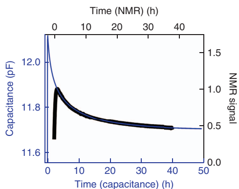
Figure 3 | Comparison with NMR data. Capacitance (blue) and 1 H NMR signal (black) as a function of time, measured on the same sample batch. The origins of the capacitance and NMR time axes are defined by the temperature jump.
