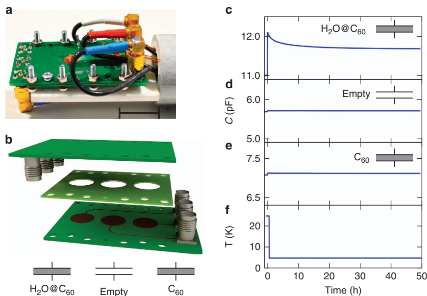
Figure 2 | Detection of ortho-para conversion in H 2 O@C 60 . (a) Photograph and (b) exploded view of the sample cell consisting of two printed circuit boards (PCBs, green) and a 210 \mu\text{m} thick G10 spacer used to centre the sample pellets between the electrodes of the two PCBs, forming three independent capacitor cells. Scale bar length in a is 2 cm. Following a temperature jump from 25 to 5 K at the time origin, the capacitance of the three cells is measured as a function of time. (c) The capacitance of the cell loaded with H 2 O@C 60 decreases monotonically due to ortho-para conversion. The capacitances of (d) the empty cell and (e) the cell loaded with C 60 change slightly as the temperature is changed, but are constant after the temperature jump. The temperature measurement is shown in f .
