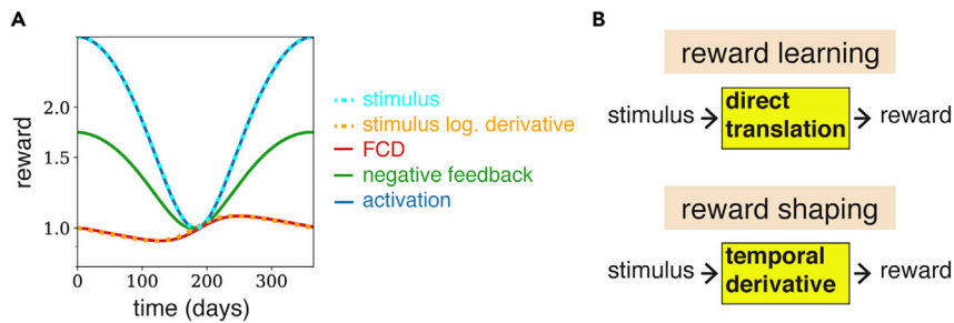
Figure 4. FCD outputs the logarithmic derivative of the input, and therefore provides a physiological implementation of potential-based reward shaping
