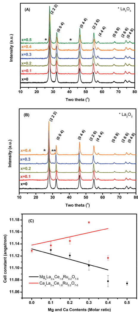
Fig. 1 Phase identification of M_x\text{La}_{2-x}\text{Ce}_{1.8}\text{Ru}_{0.2}\text{O}_{7-\delta} ( M = \text{Mg}, \text{Ca} ): (A) powder X-ray diffraction of MLCRO0-05; (B) CLCRO0-04, and (C) cell constant refinement.
