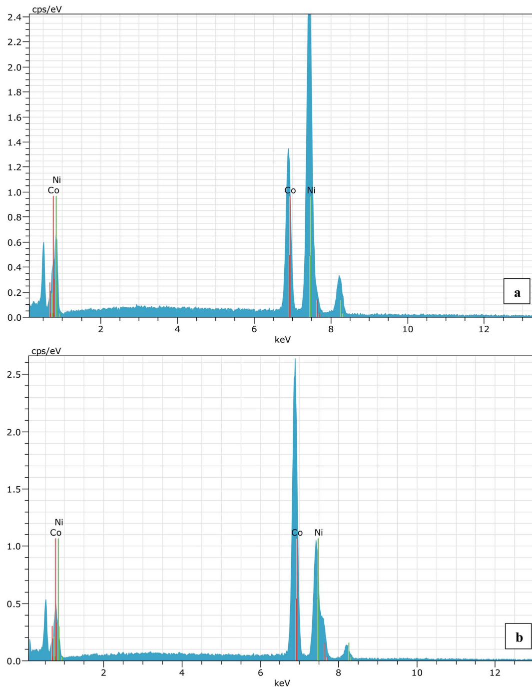
Fig. 1 (a) EDS spectrum for 30% (nominal value) Co substitution in NiO and (b) is for 70% (nominal value) Co substituted NiO sample. The average Co composition in both the cases are found to be 30.23% and 68.44%, respectively.
