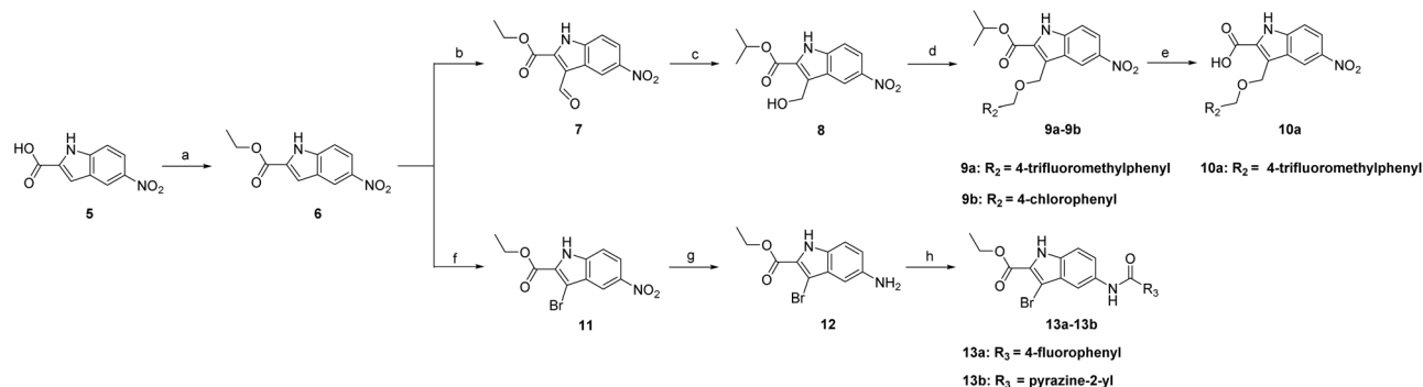
Scheme 2 Synthetic route of compounds 9a–9b , 10a , and 13a–13b . Reagents and conditions: (a) Con. \text{H}_2\text{SO}_4 , EtOH, 80 °C, 2 h, 65%; (b) \text{POCl}_3 , DMF, rt–50 °C, 4 h, 95%; (c) \text{Al}(\text{O}-i\text{-Pr})_3 , i\text{-PrOH} , 60 °C, 5 h, 80%; (d) 4-(trifluoromethyl)benzyl alcohol or 4-chlorobenzyl alcohol, \text{K}_2\text{CO}_3 , DMF, rt, 3–5 h, 79–86%; (e) NaOH, MeOH, \text{H}_2\text{O} , 80 °C, 2 h, 43%; (f) NBS, DMF, rt 4 h, 85%; (g) \text{SnCl}_2 \cdot 2\text{H}_2\text{O} , EtOAc, 80 °C, 3 h, 48%; (h) 4-fluorobenzoic acid or pyrazine-2-carboxylic acid, DMAP, EDAC, THF, rt, 3–5 h, 78–82%.
