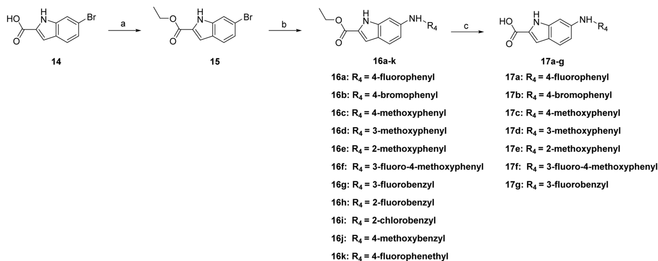
Scheme 3 Synthetic route of compounds 16a–16k and 17a–17g . Reagents and conditions: (a) Con. \text{H}_2\text{SO}_4 , EtOH, 80 °C, 2 h, 82%; (b) substituted anilines, benzylamines or phenethylamine, \text{Pd}(\text{OAc})_2 , \text{Cs}_2\text{CO}_3 , Xphos, 1,4-dioxane, 110 °C, 2–4 h, 63–82%; (c) NaOH, MeOH, \text{H}_2\text{O} , 80 °C, 1–3 h, 35–50%.
