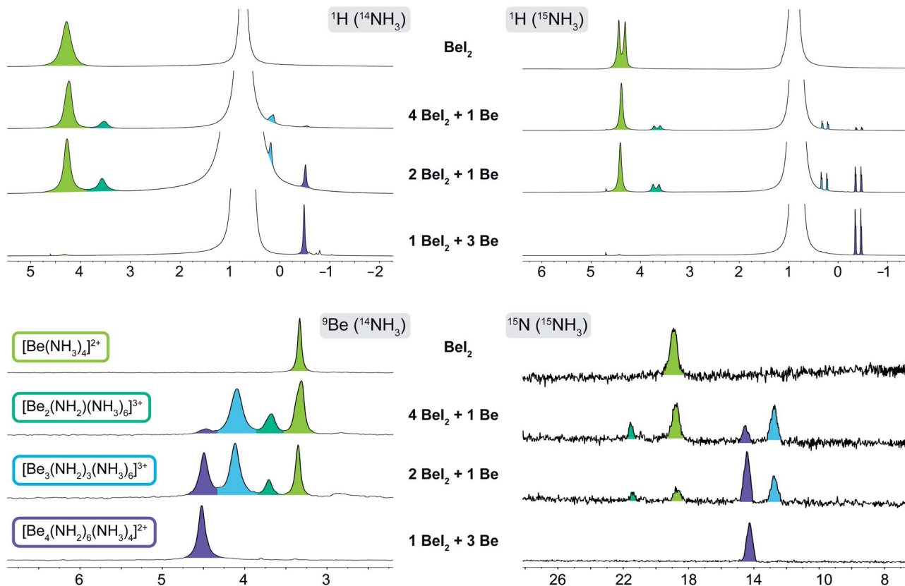
Fig. 3 ^1\text{H} , ^9\text{Be} & ^{15}\text{N} NMR spectra of four Be/ \text{Be}_{12} mixtures in liquid ^{14}\text{NH}_3 and ^{15}\text{NH}_3 respectively. Species are assigned via color code. Chemical shift \delta is given in ppm.
