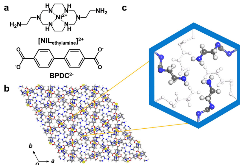
Figure 1. (a) Synthetic strategy, and (b,c) the structure ( ab plane) of a covalently alkylamine-tethered MOF ( \text{MOF}_{\text{NH}_2\text{-as}} ). (Colour scheme: Ni, yellow; C, grey; O, red; N, blue).
