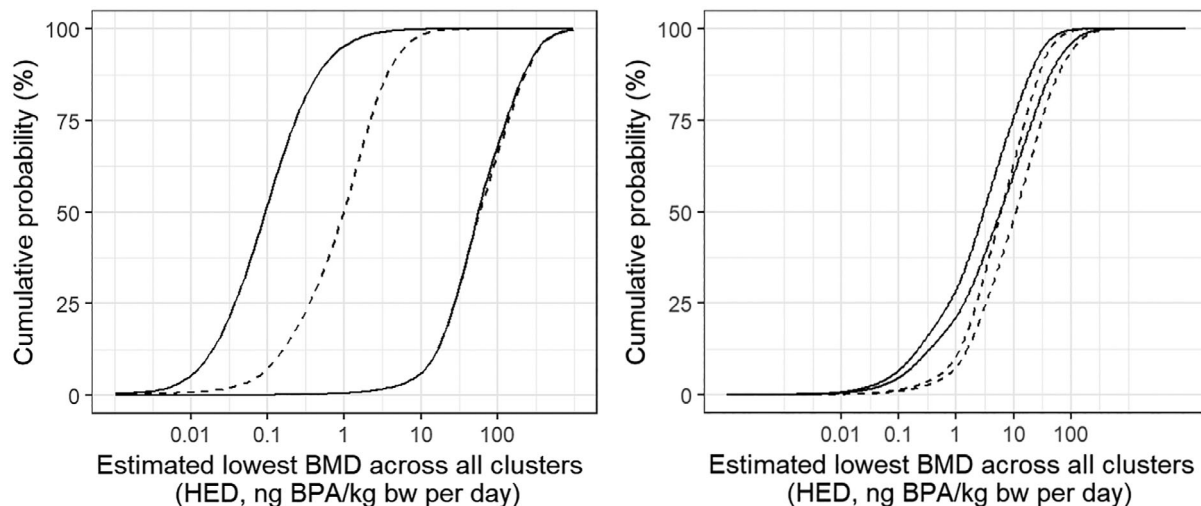
Figure D.12: Effect of including (solid curves) or excluding (dashed curves) allergic lung inflammation on the enveloped cpfs (left-hand graph) and averaged cpfs (right-hand graph) for the estimated lowest BMD across all the assessed clusters. Lower and upper bounds are shown for each cpf. See text for further explanation
