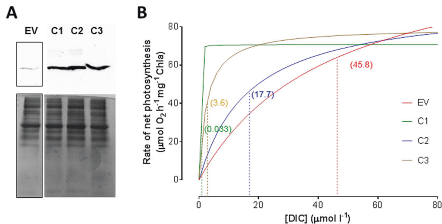
Fig. 3 LCIP63 overexpression and effect on photosynthesis in T. pseudonana . a Western blot against LCIP63 (upper) and SDS-PAGE to verify protein loading (lower) for control cells and three LCIP63-overexpressing clones. b Rate of net photosynthesis versus concentration of DIC. EV corresponds to the clone transformed with an empty vector; C1, C2, C3, to clones 1, 2, and 3 overexpressing
