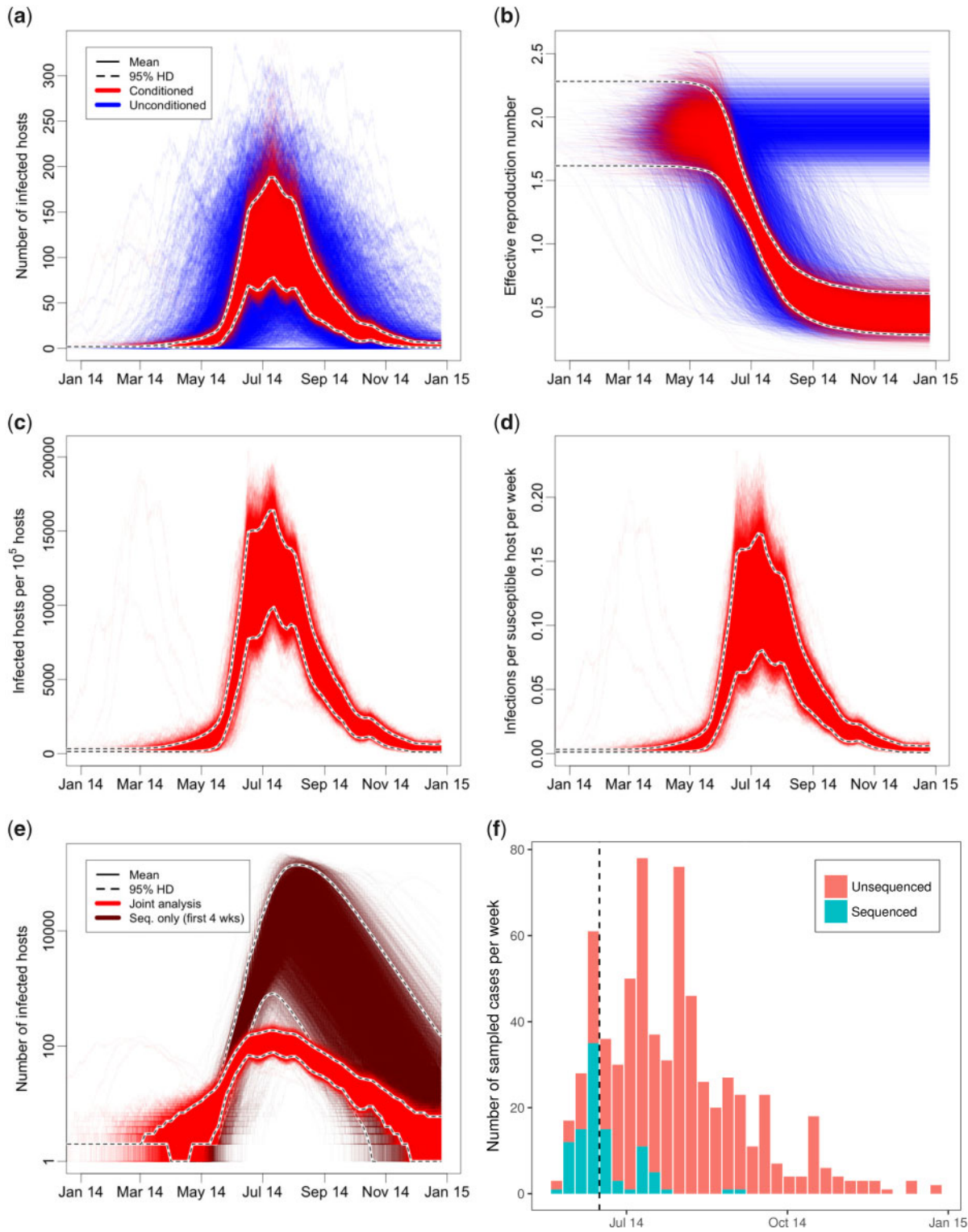
FIG. 6. (a, b) Jointly inferred posterior distributions (red) and unconditioned simulated distributions (blue) for (a) infected host count and (b) effective reproduction number during the Kailahun EVD outbreak. (c) Posterior distribution of infected host count per 10^5 hosts (prevalence). (d) Expected number of new EVD infections per susceptible host per week (incidence). (e) Comparison of inferred number of infected hosts using all data (red curves) and only the first 4 weeks of sequence data (brown curves). (f) Temporal distribution of EBOV cases used in the full analysis, both sequenced (turquoise) and unsequenced (orange). The vertical dashed line in (f) indicates the end of the 4-week period of sequence data used to infer the brown trajectories in (e).
