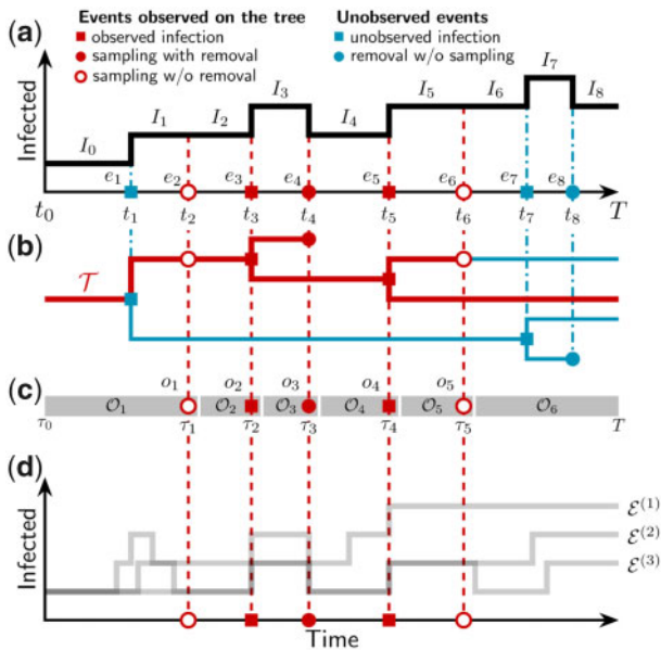
FIG. 1. The true epidemiological trajectory can be inferred from the reconstructed phylogeny. (a) The trajectory \mathcal{E} of an epidemic outbreak consists of a sequence of events (infection, sampling, and recovery) e_i at times t_i that result in a corresponding sequence of compartment occupancies such as the infectious compartment occupancies I_i . (b) The full transmission tree contains information on when infections happened and between which lineages (filled squares) and when individuals were removed (filled circles). The sampled transmission tree \mathcal{T} represents a subset of the full tree (red). The rest of the transmission tree is unobserved (blue). (c) The time ordered observations \mathcal{O}_j consist of the events o_j seen on the tree (infection, sampling with removal, and sampling without removal) at times \tau_j , combined with the number of lineages on the sampled tree in the intervals immediately before each of these events. (d) There is an ensemble of trajectories \mathcal{E}^{(1)}, \mathcal{E}^{(2)}, \dots that are compatible with the sampled transmission tree. Note that the sampled transmission tree contains only a subset of the events represented by the full tree and true trajectory \mathcal{E} , and each of these “observed” events must be present in every compatible trajectory.
