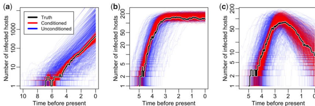
FIG. 4. Inference of prevalence dynamics from sequence data simulated under (a) linear birth–death, (b) stochastic SIS, and (c) stochastic SIR model. Samples from the posterior of the prevalence trajectory are shown in red, whereas the black line represents the truth. The blue lines are prevalence trajectories simulated from the posterior samples of the compartmental model parameters.
