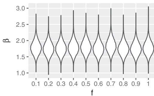
FIG. 3. Marginal posteriors for the infection rate as a function of the fraction f of samples regarded as “sequenced” when no data besides the sampling times are available. The invariance of this distribution with respect to f shows that the treatment of unsequenced samples is consistent with the treatment of sequenced samples.
