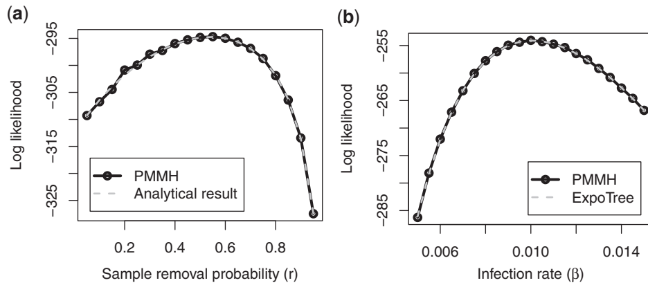
FIG. 2. Comparison between values of the phylodynamic likelihoods computed using the PMMH algorithm with those calculated using other approaches: (a) likelihood of r under the linear birth–death model from PMMH compared with the analytical result (Stadler 2010) and (b) likelihood of \beta under the stochastic SIS model from PMMH compared with a numerical result from ExpoTree (Leventhal et al. 2014).
