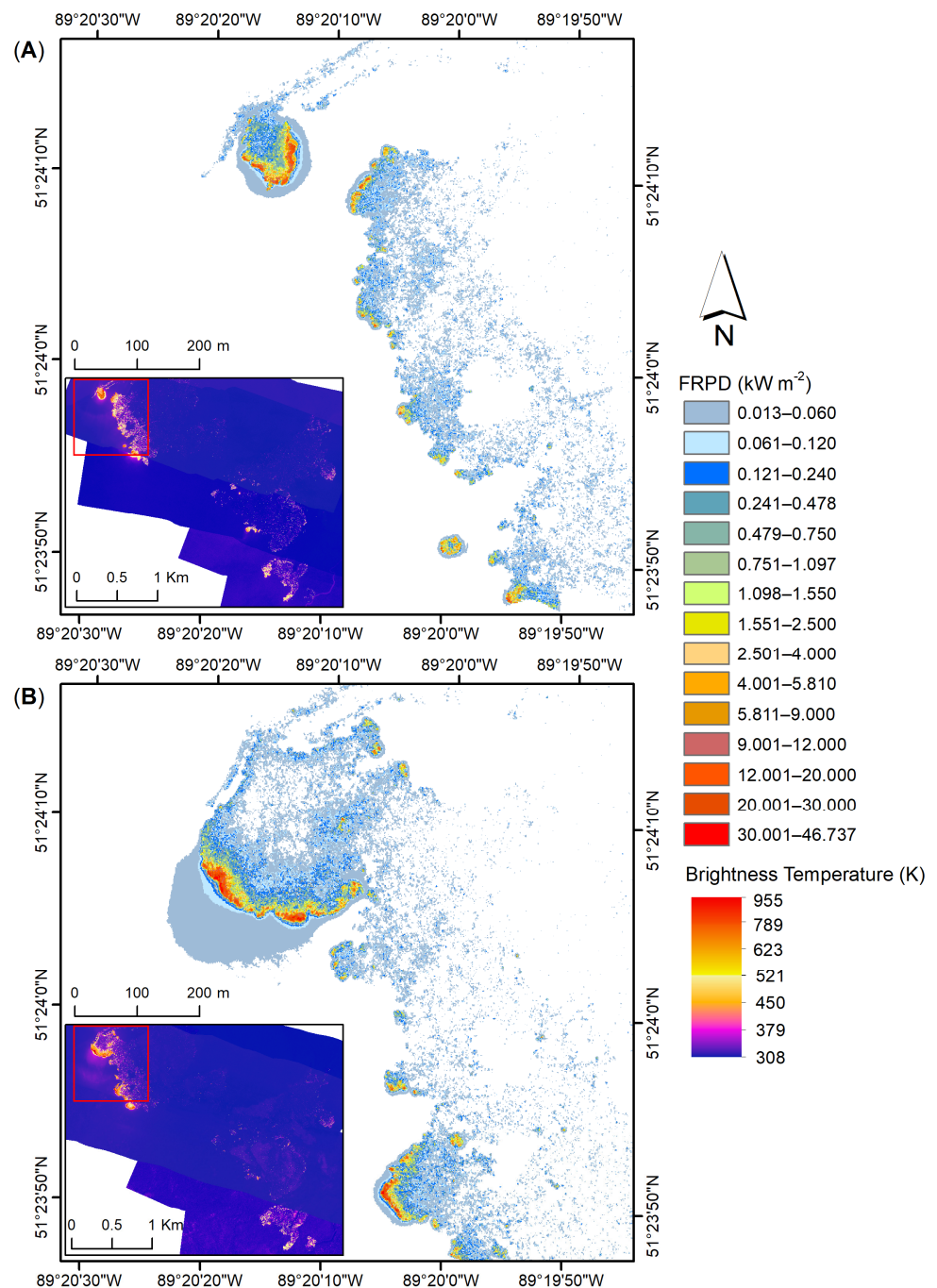
Figure 15. Example of FRPD ( \text{kWm}^{-2} ) captured over FL-05 during both (A) nighttime flight, FL-03, on 2 August, and, (B) daytime flight, F-04, on 3 August, during the 2017 campaign over the SLK-37 site. Calculated FRPD of the 1.4 ms, 0.3 ms, 0.04 ms, and 0.0021 ms integration times superimposed based on the set thresholds (Section 3.3). Overall inset area shown in brightness temperature (K) as a reference.
