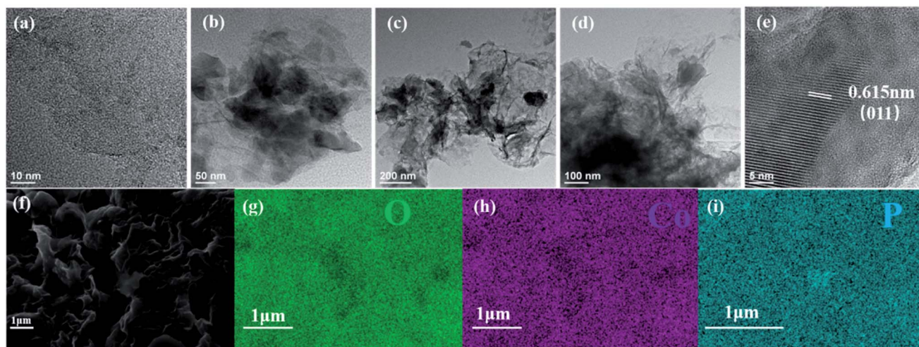
Fig. 2 (a) TEM images of 3D RGO, (b–e) TEM and HRTEM images of Co(PO 3 ) 2 -3D RGO, (f–i) SEM images and Co, P, and O element mapping images of Co(PO 3 ) 2 -3D RGO.
