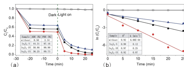
Fig. 9 Photodegradation of RhB without In_2S_3 ( \square ), In_2S_3 -5 ( \blacksquare ), In_2S_3 -10 ( \bullet ), In_2S_3 -15 ( \blacktriangle ) (a) and the corresponding plots of \ln(C_t/C_0) versus irradiation time (b), the insert tables to (a) and (b) show adsorption efficiency (ADE), photodegradation efficiency (PDE) and correlation coefficient ( R^2 ), rate constant ( k ) of different samples.
