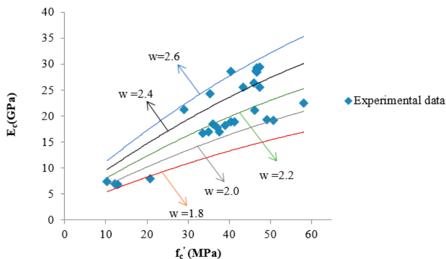
Figure 4. The suggested relationship, Equation (8), between compressive strength and elastic modulus of CFGPC applied with different density values.
