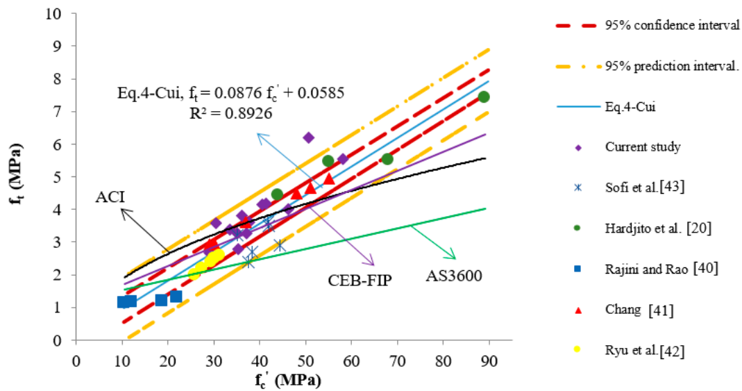
Figure 2. Relationships between splitting tensile strength and compressive strength of CFGPC (AS3600, ACI 363R-92, CEB-FIP, proposed Equation (4), etc.).
