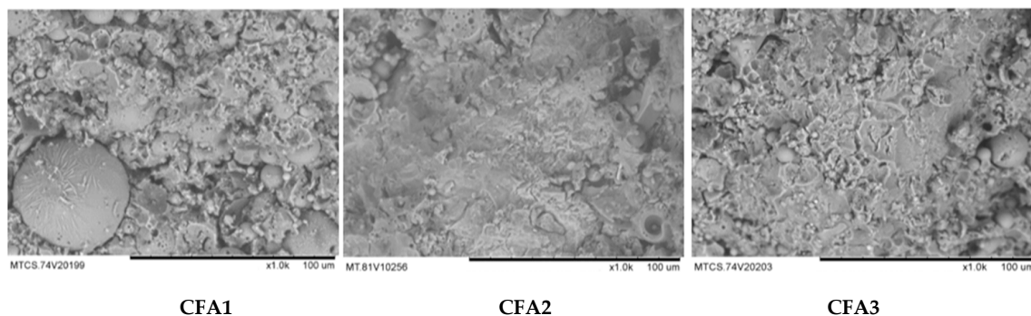
Figure 1. SEM photos for CFGPC made from CFA1, CFA2 and CFA3.
