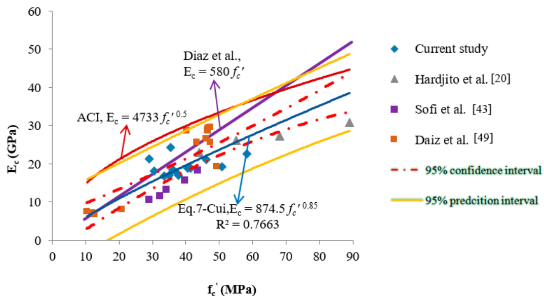
Figure 3. Relationships between elastic modulus and compressive strength of CFGPC (ACI318-14, Diaz et al., proposed Equation (7), etc.)
