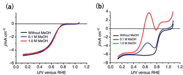
Fig. 3 j vs. U curves for (a) 12 wt% Pt-CTF and (b) 20 wt% Pt/C in 0.5 M H 2 SO 4 saturated with dissolved O 2 . The methanol concentration: (black) 0 M, (blue), 0.1 M and (red) 1 M. Reproduced from ref. 38 under the CC BY 4.0 license.
