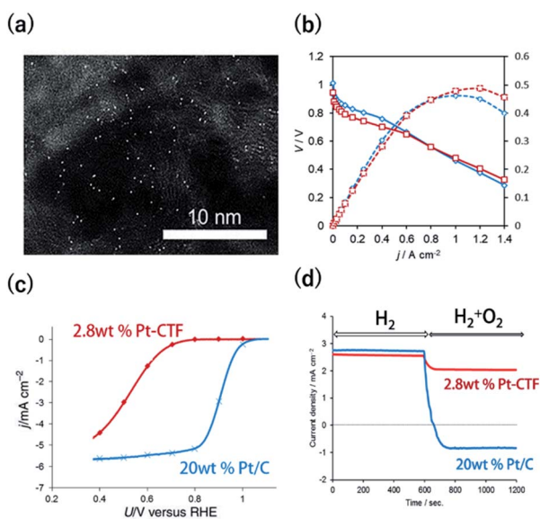
Fig. 2 (a) A representative HAADF-STEM image of a Pt-CTF. (b) j - V curves (solid line) and j -power density curves (dashed line) for MEAs. Anode catalysts: (red) 2.8 wt% Pt-CTF ( 0.020 \text{ mg}_{\text{Pt}} \text{ cm}^{-2} ) and (blue) 20 wt% Pt/C ( 0.10 \text{ mg}_{\text{Pt}} \text{ cm}^{-2} ). (c) j vs. U curves for the ORR at a sweep rate of 10 \text{ mV s}^{-1} and a rotation rate of 1600 rpm in 0.1 M \text{HClO}_4 at 25 °C. Catalysts: (red) 2.8 wt% Pt-CTF, (blue) 20 wt% Pt/C. (d) Current vs. time curves for (red) 2.8 wt% Pt-CTF and (blue) 20 wt% Pt/C (0.6 V vs. RHE). The input gas was altered at 600 s from pure \text{H}_2 to a \text{H}_2/\text{O}_2 mixed gas ( \text{H}_2 : \text{O}_2 = 50 : 50 ). Reprinted in part with permission from ref. 46. Copyright 2016 John Wiley and Sons.
