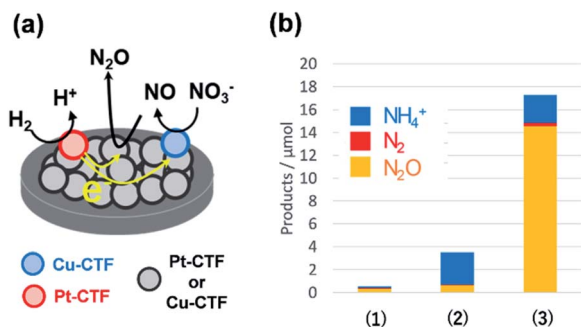
Fig. 7 (a) Local-cell catalyst composed of the Cu-CTF and Pt-CTF. (b) \text{NO}_3\text{RR} yields on (1) the Cu-CTF, (2) Pt-CTF, and (3) Cu-CTF and Pt-CTF (the local-cell catalyst) in 0.1 M \text{HClO}_4 with 0.1 M \text{Na}^{15}\text{NO}_3 under \text{H}_2 gas. Reproduced in part with permission from ref. 99. Copyright 2018 American Chemical Society.
